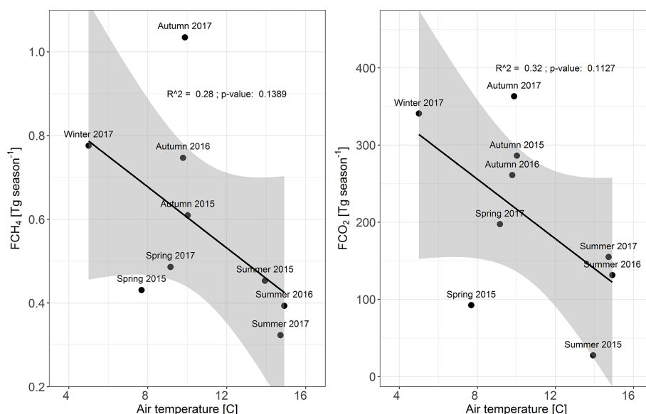
Figure 12. Seasonal budgets of CH 4 and CO 2 as a function of mean UK air temperature derived from ca. 250 synoptic stations (source: Met Office, 2018). The shaded area represents the 95 % confidence intervals of the linear regressions.
