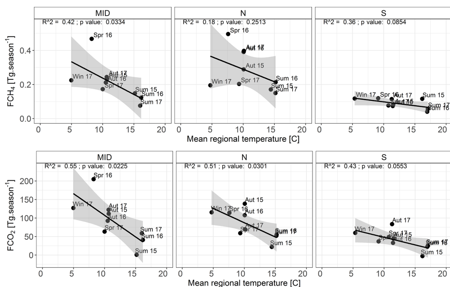
Figure 13. Seasonal fluxes of CH 4 and CO 2 estimated by mass balance from concentration measurements on board the ferry as a function of mean regional air temperature (source: Met Office, 2018). The data are presented for three latitudinal regions denoted MID, N, and S. The MID region spans the latitude range 52.8–54.2° N, N spans 54.2–56.1° N, and S spans 52.0–52.8° N. The shaded area represents the 95 % confidence intervals of the linear regressions.
