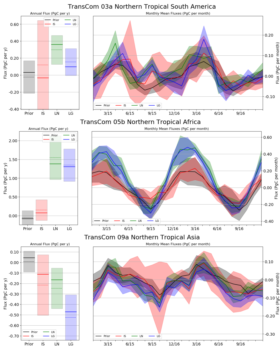
Figure 5. As in the right column of Figure 2, but for selected terrestrial regions in the northern tropics on different continents.
