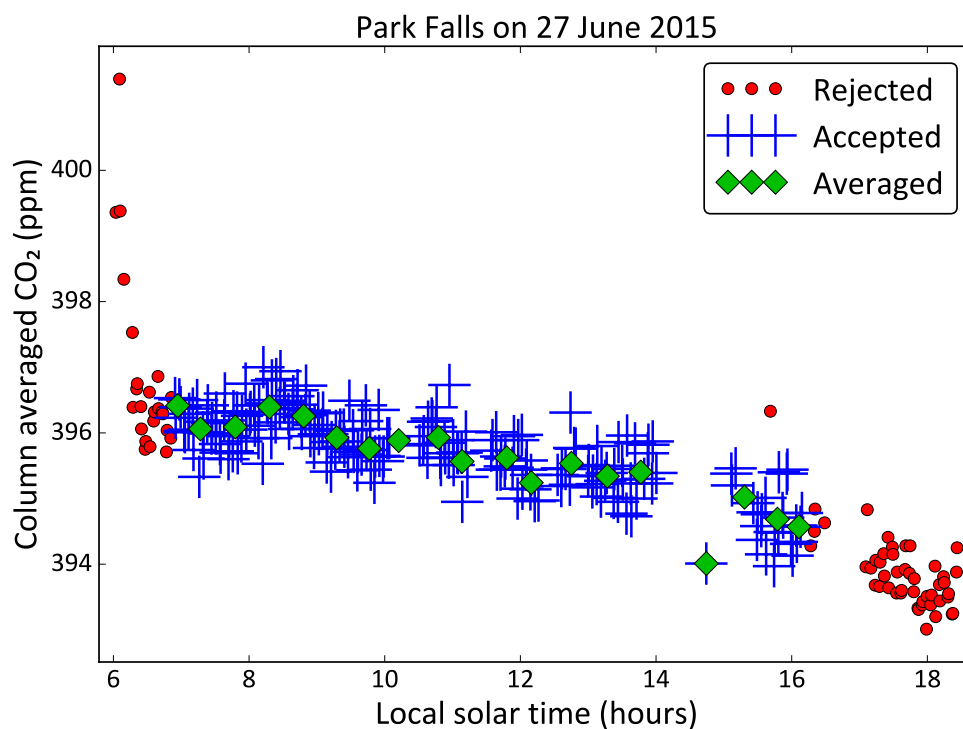
Figure C1. An example of TCCON X_{\text{CO}_2} retrievals at Park Falls on June 27, 2015. Red circles denote retrievals that were rejected by the outlier filter, SZA filter and TCCON flagging, while blue plus signs denote retrievals that passed those filters. Green diamonds denote the 30 minute averages of the accepted retrievals that were eventually used by the modelers for this study.
