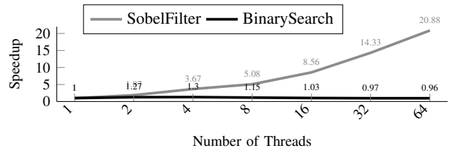
Fig. 10: Increasing the number of host simulation threads yields vast performance improvements for certain benchmarks.
