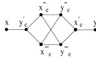
FIG. 5. Transformation of G where edge e = [x, y] is precolored into G^* .
