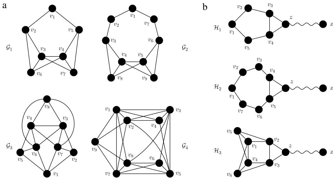
Fig. 1. Forbidden induced subgraphs for fractionally co-strongly perfect graphs. (a) The graphs \mathcal{G}_1, \mathcal{G}_2, \mathcal{G}_3, \mathcal{G}_4 . (b) Hefts \mathcal{H} that are combined to construct skipping ropes.
