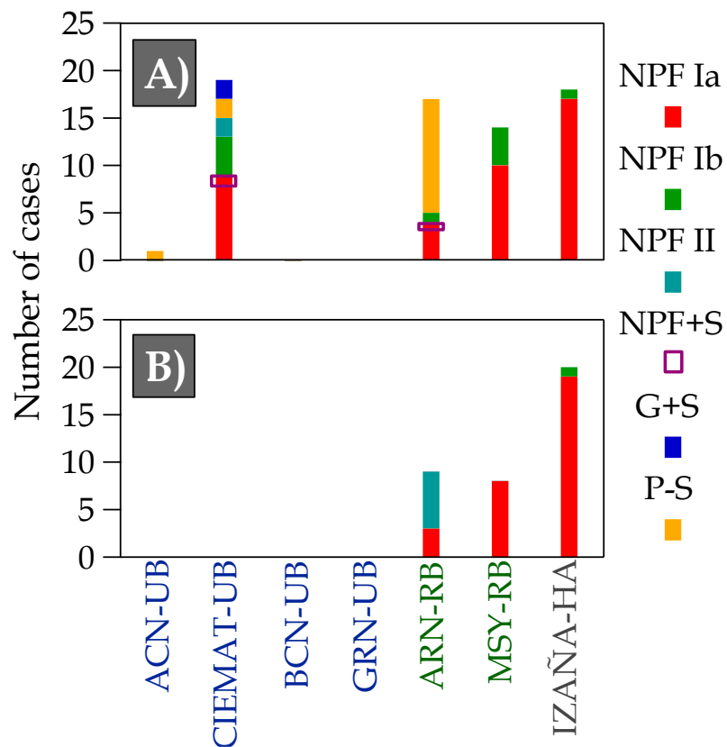
Fig. 6. Number of NPF and aerosol particle shrinkage events observed during: A) warm REDMAAS field campaign and B) cold REDMAAS field campaign. For NPF events, NPF Ia refers to clear and strong NPF events, NPF Ib refers to NPF events with a less pronounced growth than NPF Ia and NPF II refers to NPF events with a growth and formation rate poorly defined. In the case of aerosol particle shrinkage events, NPF+S refers to shrinkage occurs after an NPF, G+S refers to shrinkage occurs after an aerosol growth process and P-S refers to a shrinkage process only. For more detailed information on categorization of NPF and aerosol particle shrinkage events, see Table 1 .
