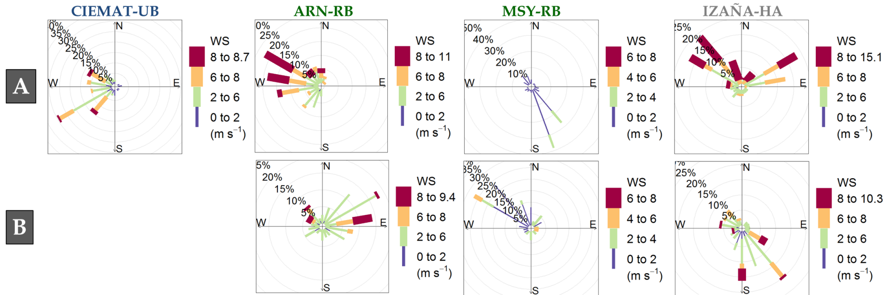
Fig. S7. Wind rose showing wind speed and direction statistics during the NPF events in CIEMAT-UB, ARN-RB, MSY-RB and IZAÑA-HA sites during the REDMAAS field campaigns: A) Warm REDMAAS field campaign and B) Cold REDMAAS field campaign.
