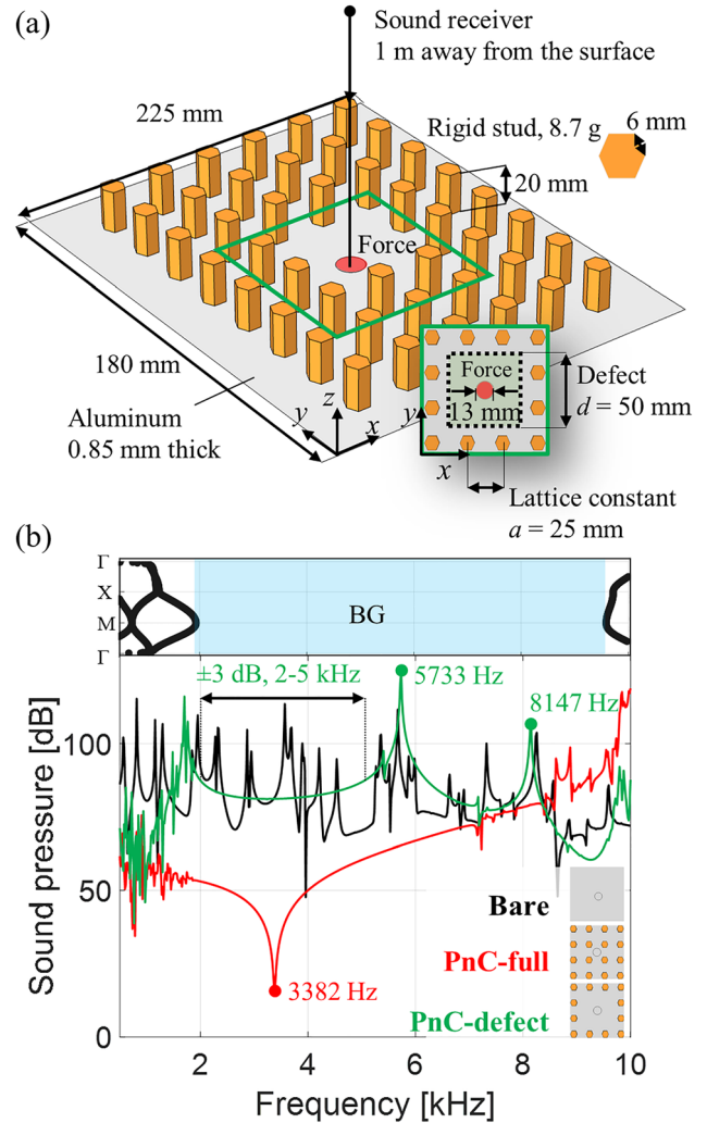
FIG. 2. (a) PnC with the defect, and (b) the sound pressure response calculated at 1 m away from the center of the surface. The reference sound pressure is 20 \mu Pa.
