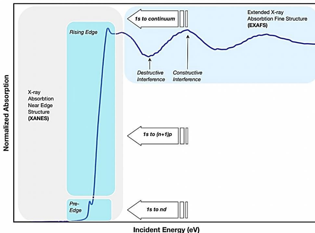
Figure 32 The areas of XAS spectrum: XANES shows in the cyan rectangles, EXAFES shown as a light blue rectangle (graphics by Munzarin/ Wikimedia Commons /CC-BY 2.0)
