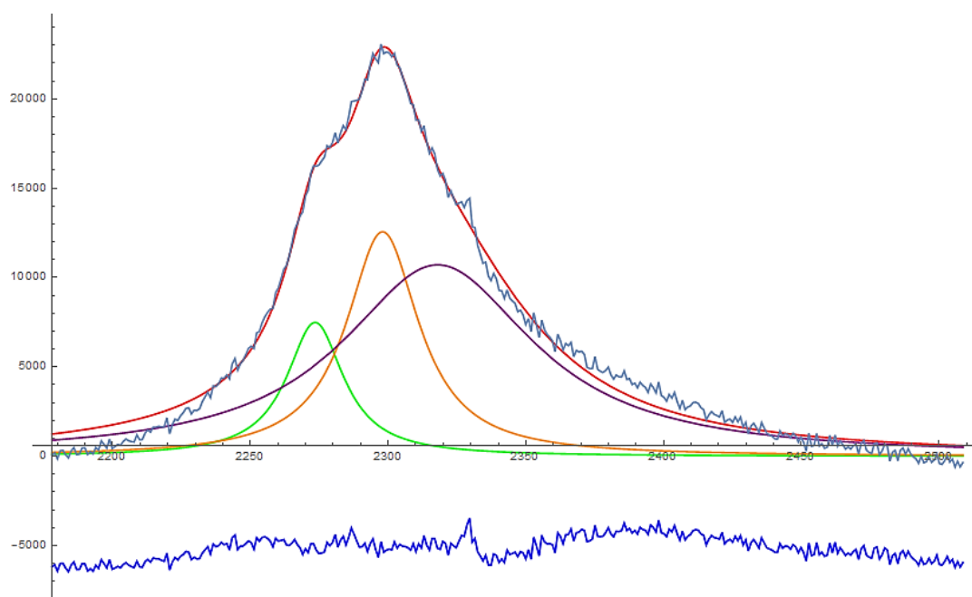
Figure 52 Raman spectrum of 30/70 wt% LiBH 4 -SiO 2 composite at 343 K (green, orange and purple lines \nu_3 , \nu_2 modes, blue line is the difference between calculated and actual spectra)
