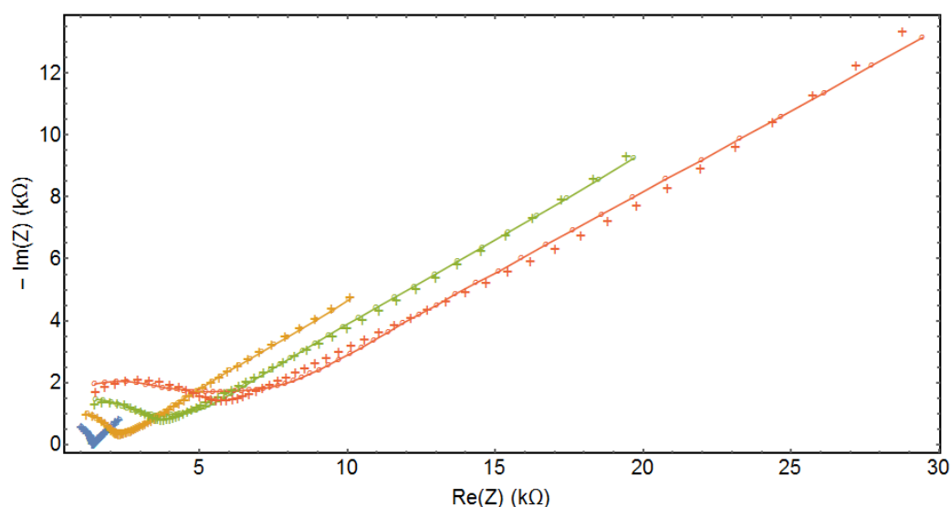
Figure 88 Every five discharge/charge cycles of a Li-S battery with their fits.
