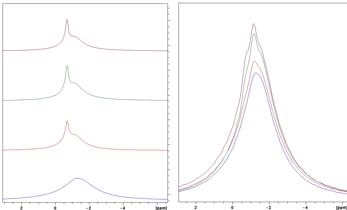
Figure 71 Left: Single pulse 7 Li resonance of 30 wt% LiBF 4 - LiBH 4 (blue) compared to 30/70 wt% LiBH 4 -SiO 2 composites at 293 K (red), 303 K (green) and 313 (purple)
