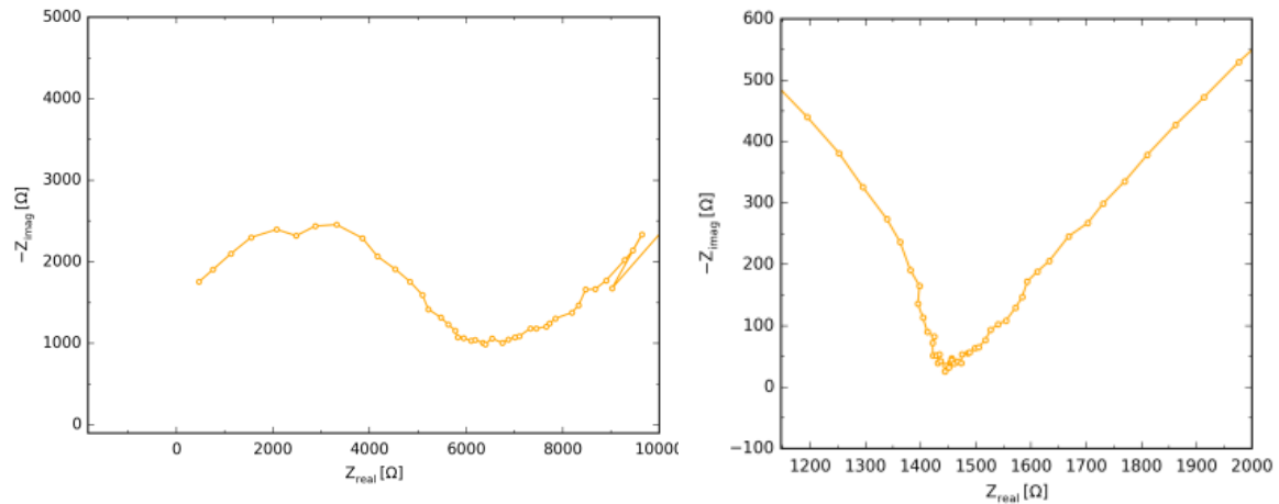
Figure 98 Impedance spectra of a fresh Li-S battery with a 1 \mu m Lipon coated C+S cathode (left) and non-coated C+S cathode (right)
