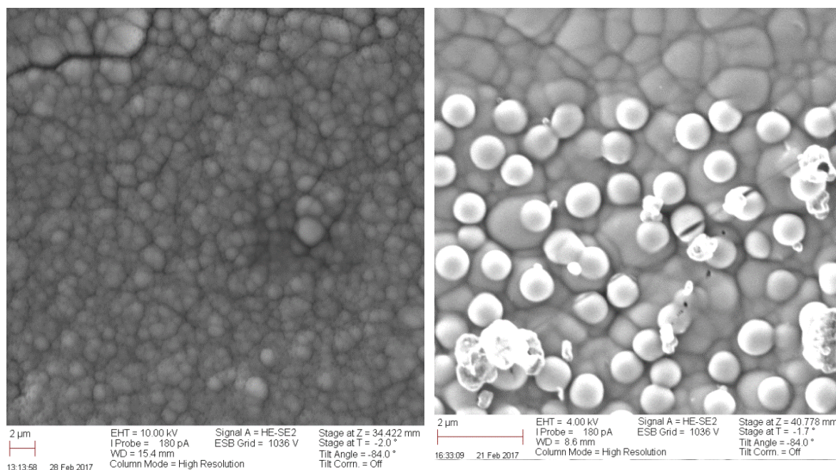
Figure 99 SEM micrograph of 1 μm Lipon-coated cathodes showing growth of bubble-like structures
