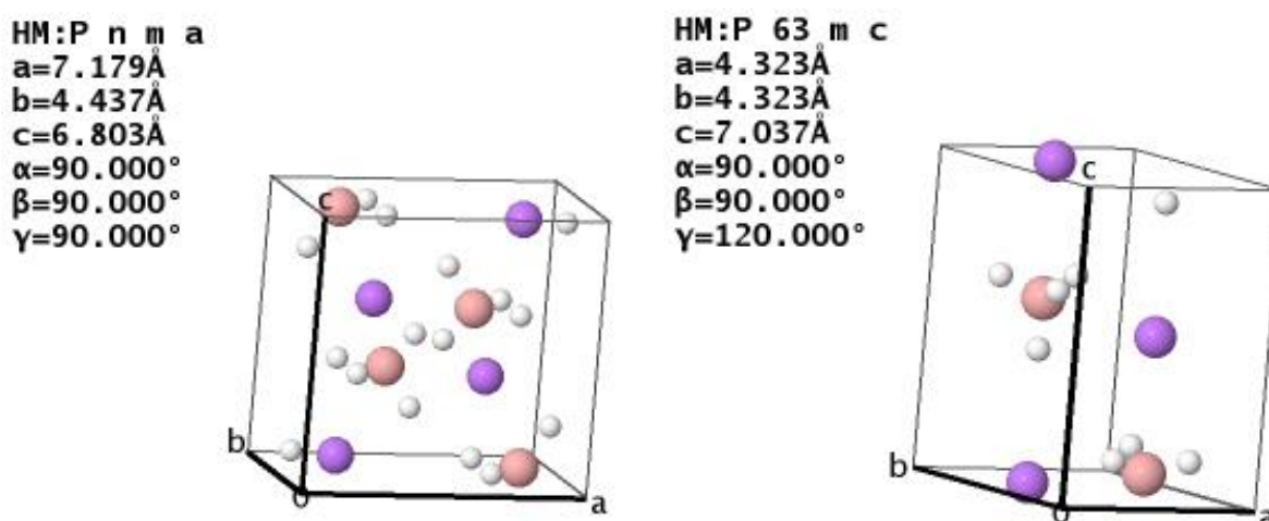
Figure 11 LiBH 4 crystal structure before ( Pnma , left) and after the phase transition ( P6 3 mc , right)
