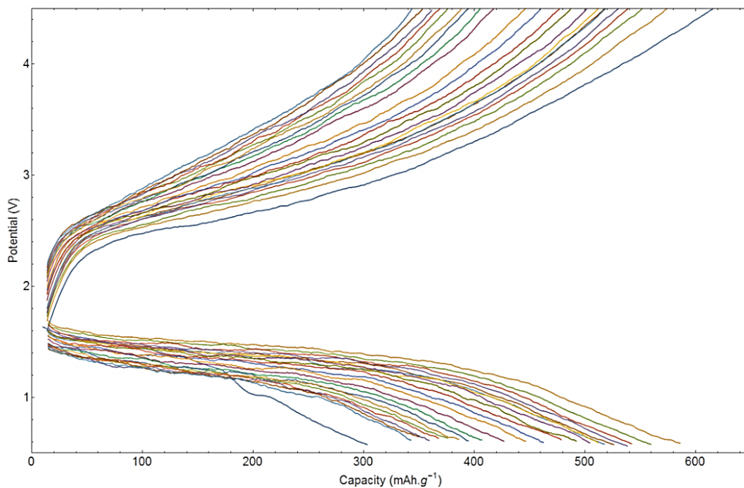
Figure 96 Discharge-charge cycles of a LiS battery with 1µm Lipon coated C+S cathode (Adapted from Lefevt, et al, 2018 116 )
