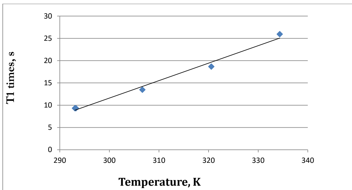
Figure 57 T1 times for pure LiBH 4 sample
