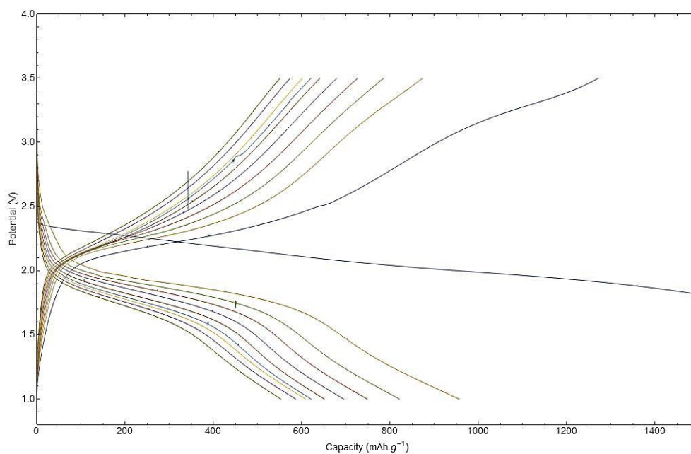
Figure 97 Discharge-charge cycles of a reference Li-S battery with C+S cathode (Adapted from Lefevt, et al, 2018 116 )
