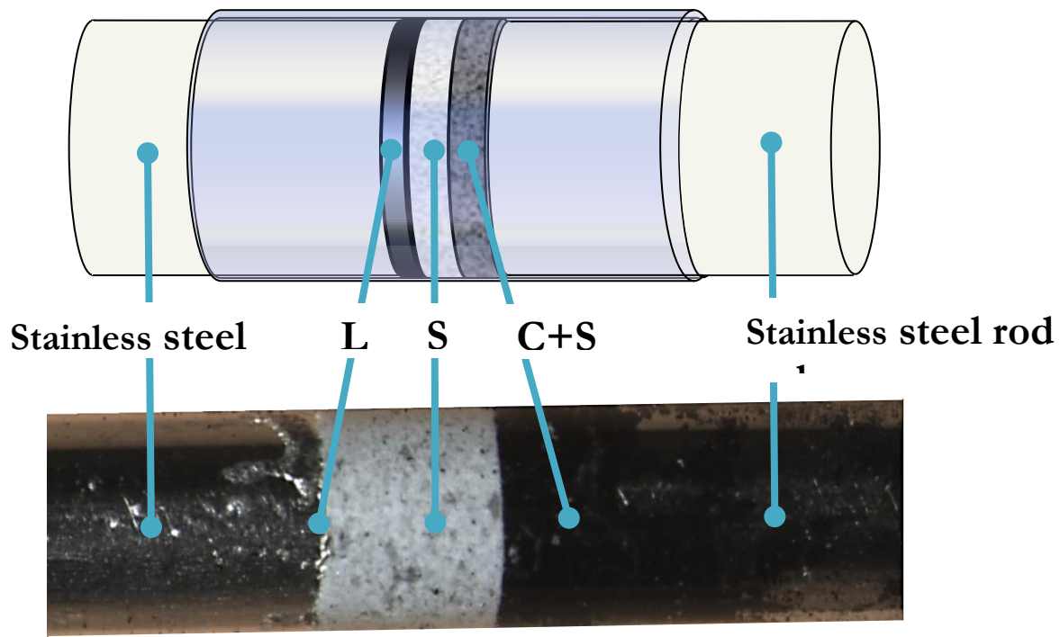
Figure 36 Schematics of a Li-S solid state battery in a quartz capillary. The gray layer is a 30 wt% LiBH 4 -SiO 2 solid state electrolyte.
