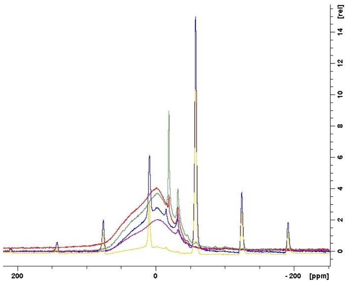
Figure A 3 11B High-power decoupling spectra 5 (yellow), 20 (blue), 30 (red), 35 (green) wt% LiBF _4 -LiBH _4 compared to pure Li _2\text{B}_{12}\text{H}_{12} (purple)
