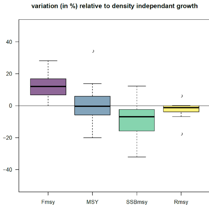
Figure 2.5.10 For 12 New England (USA Northwest Atlantic) fish stocks. Changes in Fmsy, MSY, SSBmsy and Rmsy when including density dependent growth.
