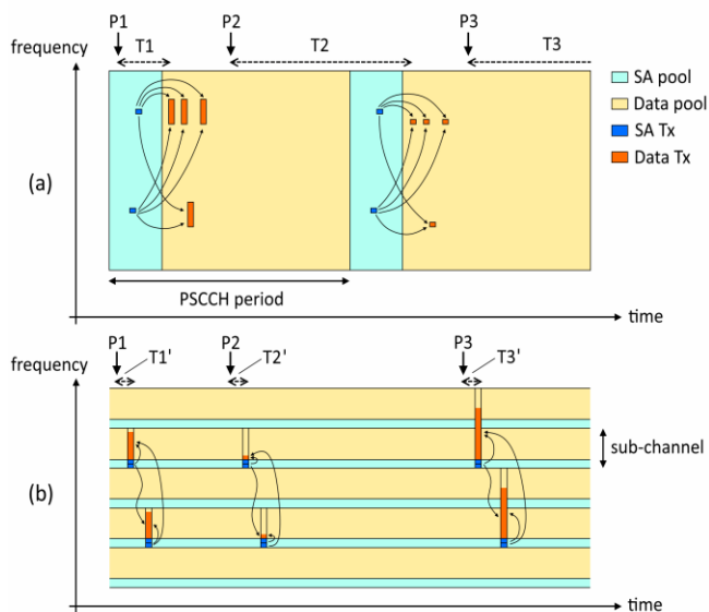
FIGURE 1. Resource allocation: a) modes 1 and 2, b) modes 3 and 4.
