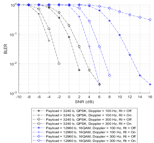
FIGURE 2. Achievable BLER vs SNR for different payload sizes, modulations, Doppler shifts and transmissions.
