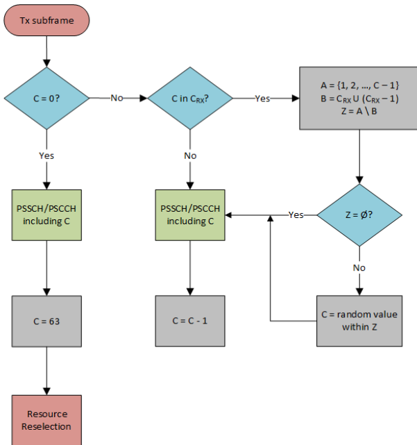
Figure 6. CLR scheduling mechanism for eV2X services.
