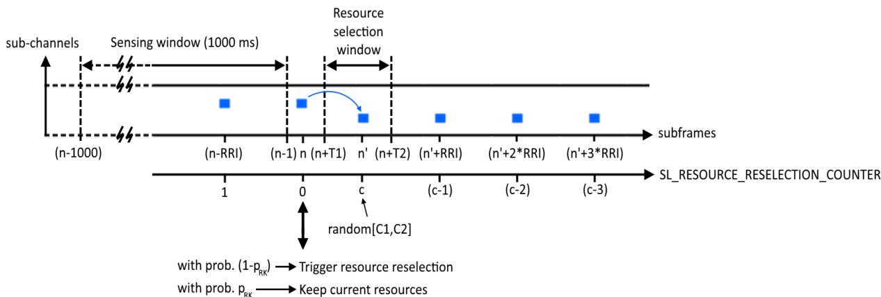
FIGURE 3. Resource reselection triggering in standardized sensing-based SPS procedure
