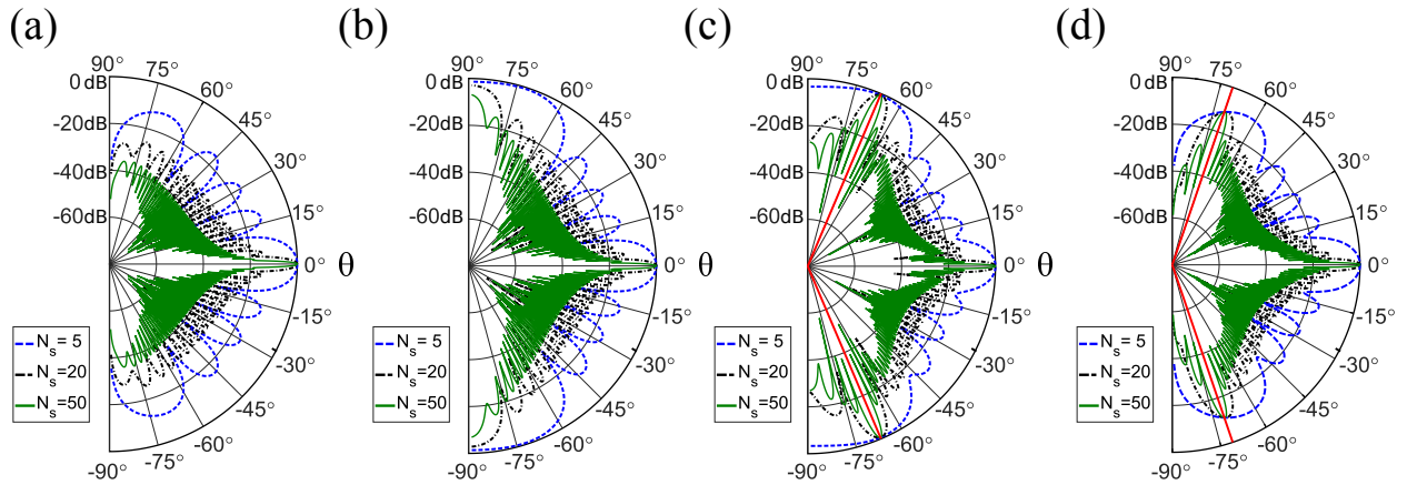
Fig. 4. Normalized radiation patterns in the y-z plane for z > 0 ( \phi = \pm 90^\circ ) of the periodic arrays of slots analyzed in Fig. 3 when: (a) \alpha = 90^\circ and a/\lambda_0 = 0.887 ; (b) \alpha = 45^\circ and a/\lambda_0 = 0.897 ; (c) \alpha = 45^\circ and a/\lambda_0 = 0.995 ; (d) \alpha = 0^\circ and a/\lambda_0 = 0.960 . The direction of the grating lobes is indicated in red. Parameters: l_s/a = 0.4 , w_s/a = 0.05 , b = 1.1a , \theta_{inc} = 0^\circ .
