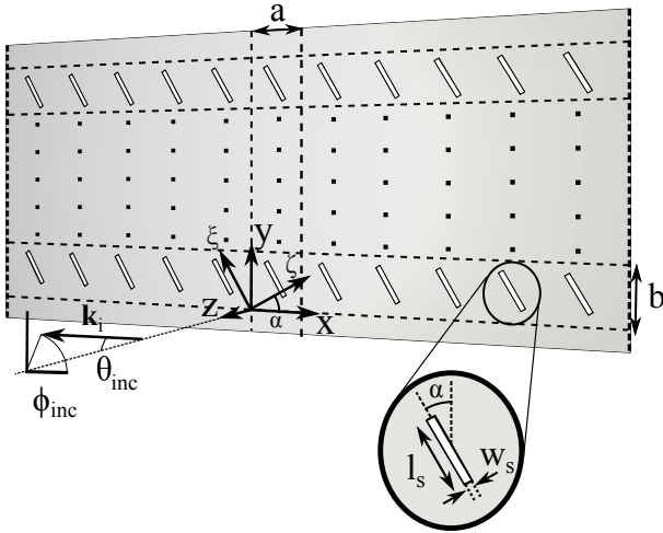
Fig. 1. Perspective view of a one-dimensional periodic array of rectangular holes. A finite number N_s of slots is assumed to be located in the y direction with a spacing b , while the number of holes in the x direction is infinite with a spacing a . The slots are rotated an angle \alpha , which also defines a new set of coordinates (\zeta, \xi) , aligned with the axes of the slots.
