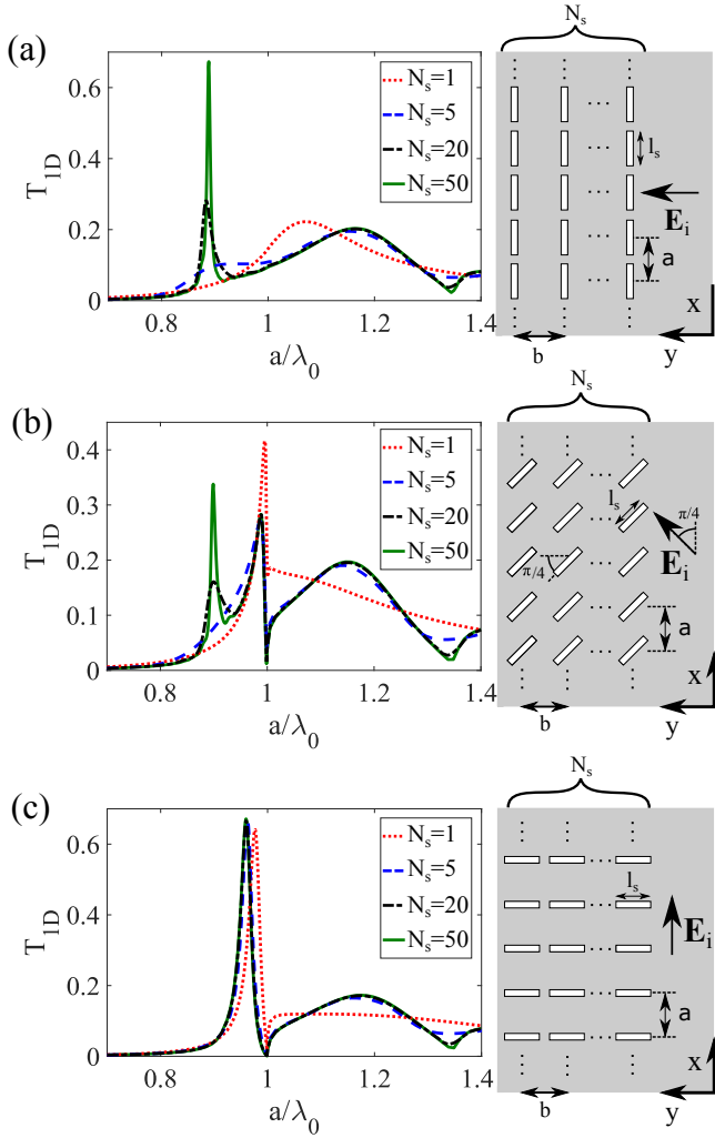
Fig. 3. Transmission coefficient of N_s parallel infinite periodic chains of slots for different values of N_s under normal incidence conditions. Results are presented for: (a) slots parallel to the periodicity direction, \alpha = 90^\circ ; (b) slots tilted an angle \alpha = 45^\circ with respect to the periodicity direction; (c) slots perpendicular to the periodicity direction, \alpha = 0^\circ . Parameters: l_s/a = 0.4 , w_s/a = 0.05 , b = 1.1a , \theta_{inc} = 0^\circ .
