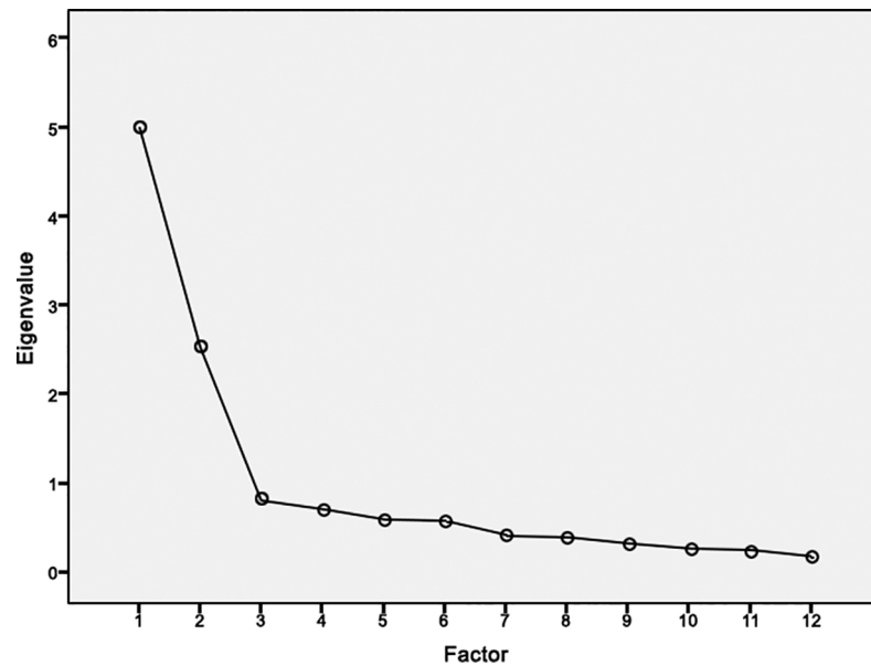
Fig 1. Scree plot.
