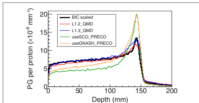
FIGURE 7 | Longitudinal profiles of the photons escaping the PMMA target having an angular acceptance of \pm 1.5^\circ using a given built-in option in Geant4 or a change in the source code. The “BIC scaled” profile refers to the BIC case scaled down to compensate the estimated overestimation of 40.2% (see Table 2 ). The naming conventions are presented in Table 3 .
