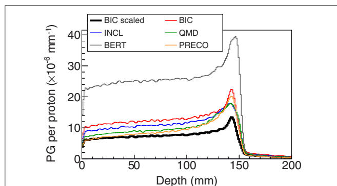
FIGURE 6 | Longitudinal profiles of the photons escaping the PMMA target having an angular acceptance of \pm 1.5^\circ . These profiles were obtained with the default models of Geant4 and the “BIC scaled,” which corresponds to the BIC case scaled down to compensate the estimated overestimation of 40.2% (see Table 2 ).
