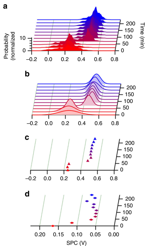
Fig. 5 Changes in surface potential contrast as the polymers de-dope. a Histograms of the surface potential contrast distribution, b Gaussian fit to each histogram, and the c mean and d width of the Gaussian fits of a film of poly(3-hexylthiophene) (P3HT) initially doped at 25 °C as it spontaneously de-dopes
