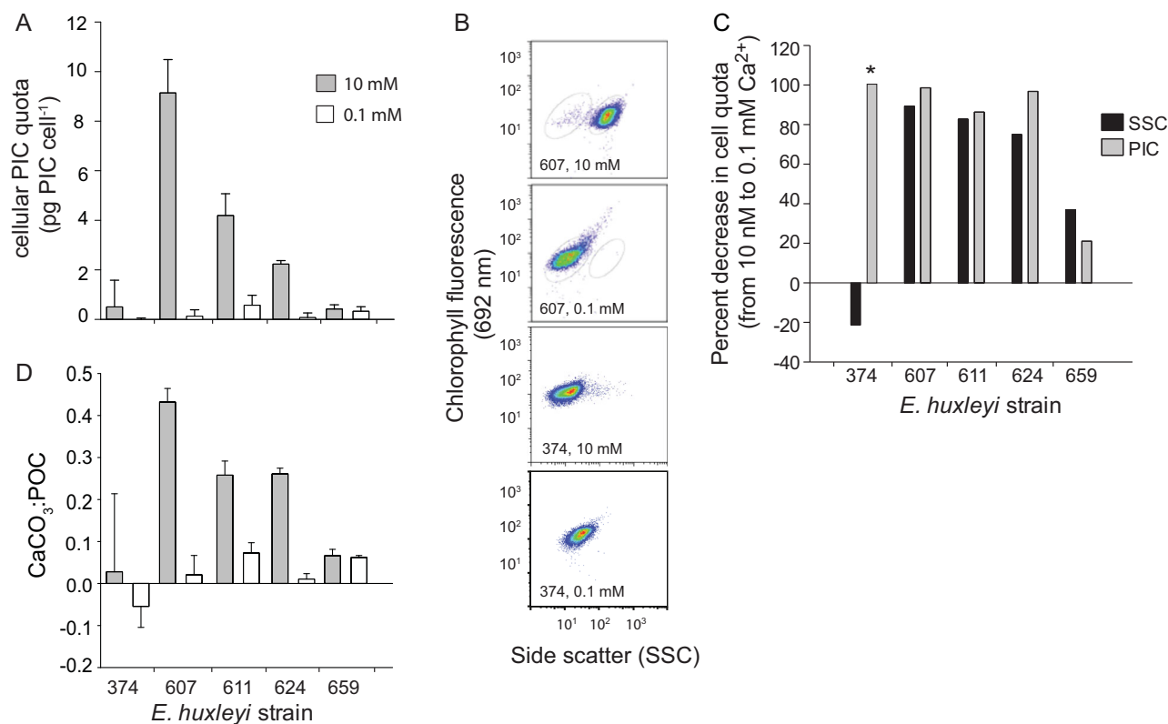
Fig. 3. Calcification state of various E. huxleyi strains grown in defined ESAW media at different \text{Ca}^{2+} concentrations. (A) Cellular PIC quota for strains grown with either 0.1 mM or 10 mM \text{Ca}^{2+} concentrations. Error bars represent the standard error ( \text{SD}/\sqrt{n} ) among triplicate measurements for one experiment; host–virus dynamics shown were representative of experiments ( n = 3 ) performed on different dates. (B) Representative flow cytometry plot showing the SSC and chlorophyll (692 nm) signals for DHB607 grown in 10 mM or 0.1 mM \text{Ca}^{2+} compared to canonical naked strain CCMP374 grown in 10 mM \text{Ca}^{2+} . Note the prominent shift to a lower SSC for DHB607 cells grown in 0.1 mM, matching that of the low SSC for CCMP374. (C) Percentage (%) decrease in both the mean cellular PIC quota and geometric mean of SSC for cells grown in 10 mM \text{Ca}^{2+} compared to those grown in 0.1 mM \text{Ca}^{2+} (asterisk for strain CCMP374 denotes that the % decrease in PIC derives from a 0 pg PIC cell -1 at 0.1 mM \text{Ca}^{2+} ). (D) \text{CaCO}_3 :POC ratios derived from the data in panel (A). We noted that growth in the ESAW artificial seawater medium at 10 mM \text{Ca}^{2+} did generally lower the total calcification state for all DHB strains compared to cells grown in f/2-Si media (Figs 1A and 3A), likely due to the presence of additional factors in seawater-based media that are required for maximum calcification. Nonetheless, these strains clearly calcified in ESAW media, maintained similar growth rates, and possessed similar cellular chlorophyll signatures, indicative of healthy cells. SEM images confirmed that there was plenty of calcite production in culture under these conditions, with the formation of fully formed coccospheres and detached coccoliths (Supporting Information Fig. S2).
