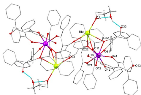
Figure 2 Representation of the X-Ray structure of 6 , [\text{Nd}(\text{Rb})(\text{tbn})_4]_2 , where hydrogen atoms have been omitted for clarity except for those on the solvent EtOH molecule.
