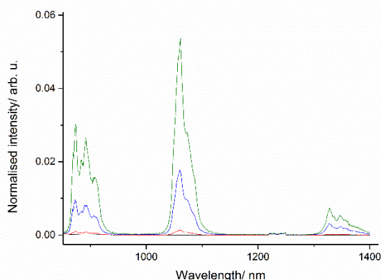
Figure 5 \text{Nd}^{3+} emission plot for complex 2 (black trace), 3 (red trace), 4 (blue trace) and 5 (green trace) with excitation wavelength at 350nm normalised at 612 nm ( \text{Eu}^{3+} emission).
