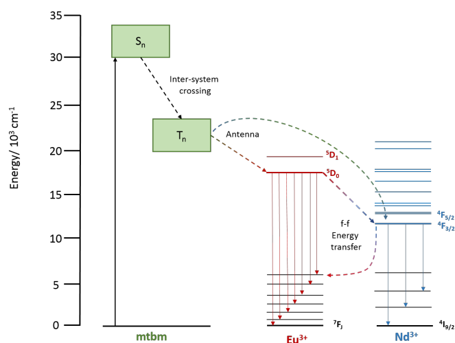
Figure 4 Energy level diagram and energy transfer occurring for the mixed complexes \{[\text{Eu}_{1-x}\text{Nd}_x(\text{Rb})(\text{mtbm})_4]_2\}_n
