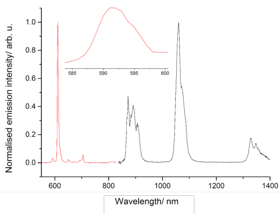
Figure 3 Normalised emission plot for [[\text{Eu}(\text{Rb})(\text{mtbm})_4]_2]_n (red trace) and [[\text{Nd}(\text{Rb})(\text{mtbm})_4]_2]_n (black trace) in the solid state, with excitation wavelength at 350nm. Inset: highlight of the splitting of the magnetic dipole transition for the Eu 3+ complex.
