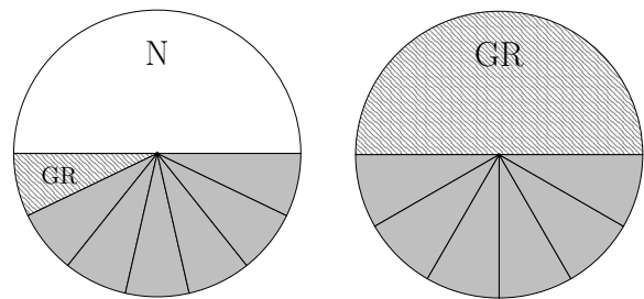
FIG. 4. Model priors. Distribution of prior probability over subhypotheses for the construction of \mathcal{O}_N^S (left) and \mathcal{O}_{\text{GR}}^{\text{GR}} (right), according to Eqs. (43) and (45) respectively. For \mathcal{O}_N^S , we assign equal weight to the \mathcal{H}_N (white) and \mathcal{H}_S (gray); as in Eq. (64), we make no a priori distinction between non-GR models (solid) and GR (hatched). For \mathcal{O}_{\text{GR}}^{\text{GR}} , we set equal prior probability for \mathcal{H}_{\text{GR}} and \mathcal{H}_{\text{nGR}} , distributing the prior equally among non-GR models, as in Eq. (66).
