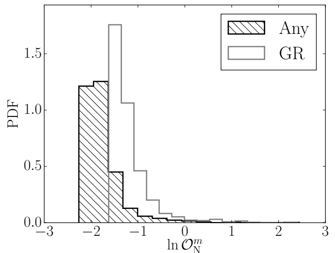
FIG. 5. Signal vs noise log-odds background distributions for any-signal and GR hypotheses. Histograms of \ln \mathcal{O}_N^S (black line, hatched) and \ln \mathcal{O}_N^{GR} (gray line) over an ensemble of 1000 simulated noise instantiations corresponding to the Crab pulsar. For each instantiation, three time series of Gaussian noise were produced using the design noise spectra of H1, L1 and V1, as outlined in Sec. IV; the data are analyzed coherently across detectors. (Note that here \ln \mathcal{O}_N^{GR} = \ln \mathcal{B}_N^{GR} , since we assign equal weight to both models.)
