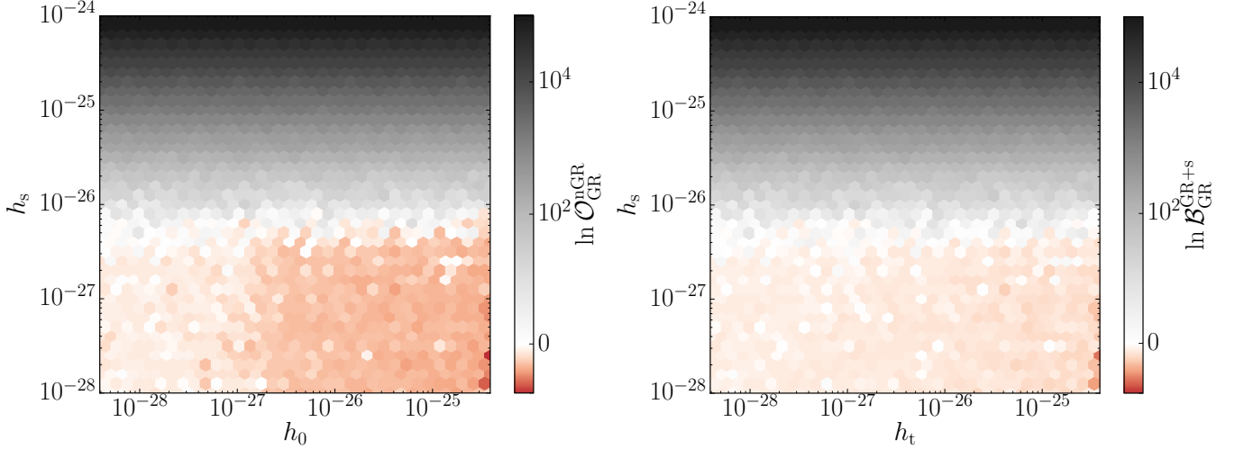
FIG. 11. Categorizing scalar-tensor injections ( \mathcal{H}_{\text{nGR}} & \mathcal{H}_{\text{GR}+\text{s}} vs \mathcal{H}_{\text{GR}} ). Log-odds comparing the non-GR and GR+s hypotheses to GR. The non-GR odds is defined in Eq. (45). Each plot was produced by analyzing 2500 instantiations of data (one time series for each detector: H1, L1 and V1) made up of Gaussian noise plus a simulated Crab-pulsar GR+s signal of the indicated tensor ( x -axis) and scalar ( y -axis) amplitudes. The color of each hexagon represents the average value of the log-odds in that region of parameter space; color is normalized logarithmically, except for a linear stretch in the (-1, 1) range.
