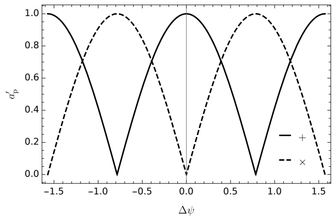
FIG. 17. Effect of changing polarization angle. Norm of the complex plus ( a'_+ , solid line) and cross ( a'_x , dashed line) weights after rotating the source by \Delta\psi in the plane of the sky, i.e. letting \psi \rightarrow \psi' = \psi + \Delta\psi ; this transformation is expressed in Eqs. (A5) and (A6). In this case, we start from a_+ = 1 , a_x = 0 and \psi = 0 .
