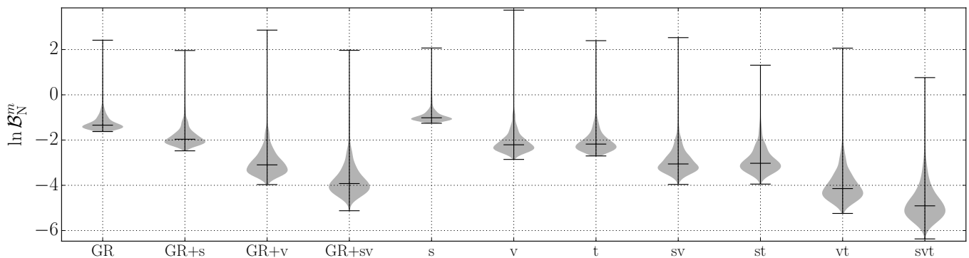
FIG. 6. Signal vs noise log-Bayes background distributions for all subhypotheses. Violin plots representing histograms of the log-Bayes of several models versus noise, computed over an ensemble of 1000 simulated noise instantiations each corresponding to H1, L1 and V1 design data prepared for the Crab pulsar; the data are analyzed coherently across detectors. The labels on the x -axis indicate which hypothesis is being compared against noise; the “GR” label indicates tensor modes parametrized by Eq. (29) with fixed \psi and \iota . Black lines mark the range and median of each distribution. (The gray histogram in Fig. 5 corresponds to the leftmost distribution here.)
