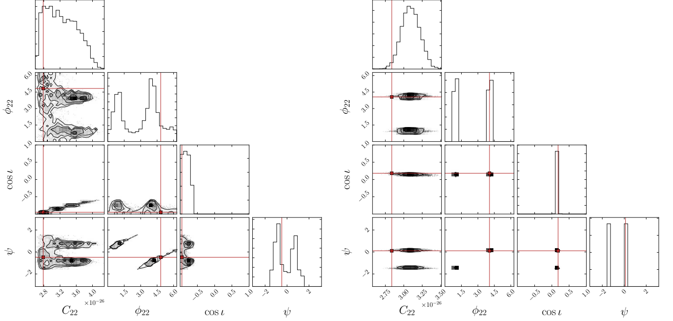
FIG. 19. Effect of inclination. Posterior PDFs for parameters of \mathcal{H}_{\text{GR}} with unfixed source orientation ( \psi, \iota ). Each panel consists of a corner plot displaying the two-dimensional posteriors for each pair of parameters as indicated by the x and y labels, with the diagonals showing a histogram of the one-dimensional PDF for each parameter. The data sets analyzed contain signals with parameters indicated by the red lines; note that C_{22} = h_0/2 is the quantity that was actually used to parametrize GR triaxial amplitudes in the code [33]. On the left, the injected signal corresponds to a face-off source ( \cos \iota \approx -1 ), making it difficult to constrain the polarization angle \psi ; on the right, the injection has similar amplitude but corresponds to an edge-on source ( \cos \iota \approx 0 ), making it easy to constrain \psi [modulo \pi/2 due to the 2\Delta\psi dependence of Eqs. (A3) and (A4)]. These plots were produced using the corner.py package [49].
