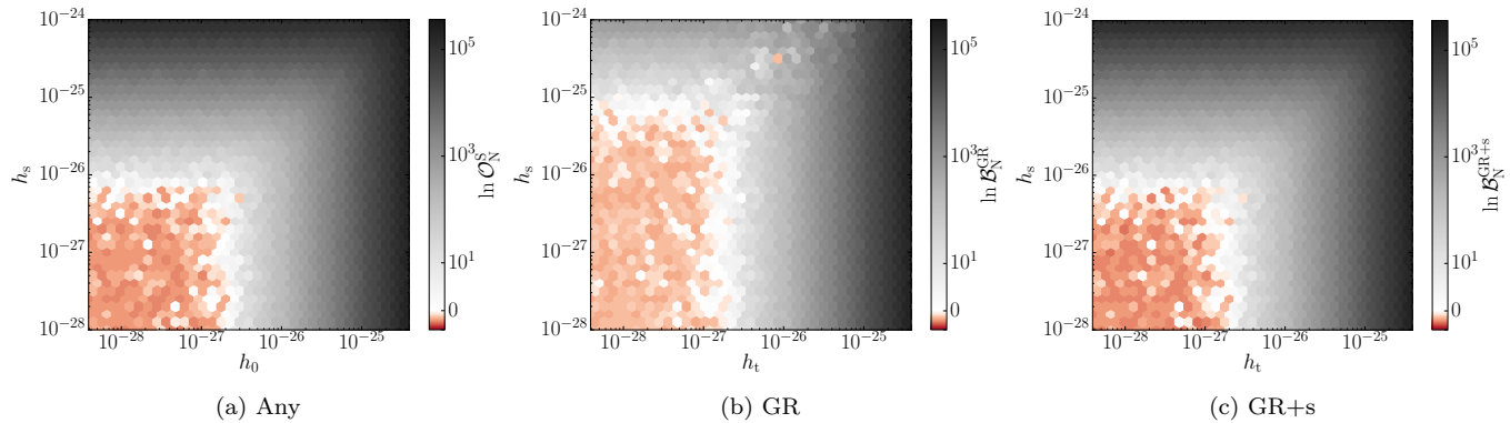
FIG. 8. Expected sensitivity to scalar-tensor injections. Log-odds of any-signal ( \mathcal{H}_S , left), GR ( \mathcal{H}_{GR} , center) and GR+s ( \mathcal{H}_{GR+s} , right) hypotheses versus noise. The any-signal odds is defined in Eq. (43). Each plot was produced by analyzing 2500 instantiations of data (one time series for each detector: H1, L1 and V1) made up of Gaussian noise plus a simulated Crab-pulsar GR+s signal of the indicated tensor ( x -axis) and scalar ( y -axis) amplitudes. The color of each hexagon represents the average value of the log-odds in that region of parameter space; color is normalized logarithmically, except for a linear stretch in the (-1, 1) range.
