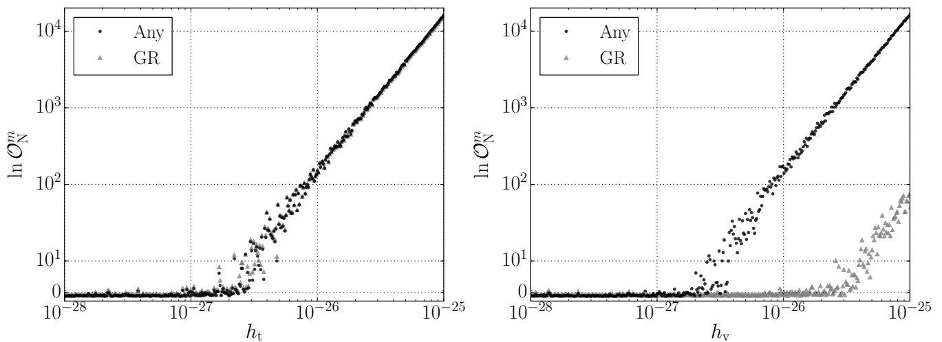
FIG. 7. Expected sensitivity to GR and vector injections. Log-odds of any-signal ( \mathcal{H}_S , black circles) and GR ( \mathcal{H}_{GR} , gray triangles) versus noise ( \mathcal{H}_N ) hypotheses, as a function of injection amplitude, for signals corresponding to both GR (left) and the vector-only model from [21] (right). The any-signal odds is defined in Eq. (43). Each of the 500 points corresponds to a data instantiation (one time series for each detector: H1, L1 and V1) made up of Gaussian noise plus a simulated Crab-pulsar signal of the indicated strength. The injections were performed with random values of the nuisance phase parameters, and the data were analyzed coherently across detectors. A logarithmic scale is used for the y -axis, except for a linear stretch corresponding to the first decade.
