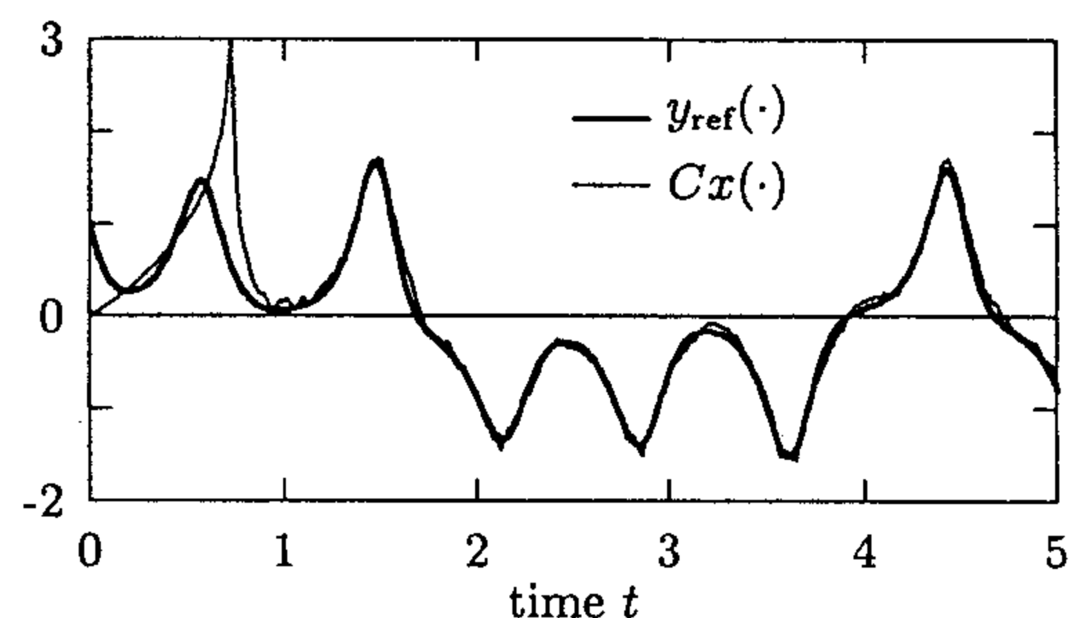
FIG. 6. Tracking behaviour in presence of noise.
