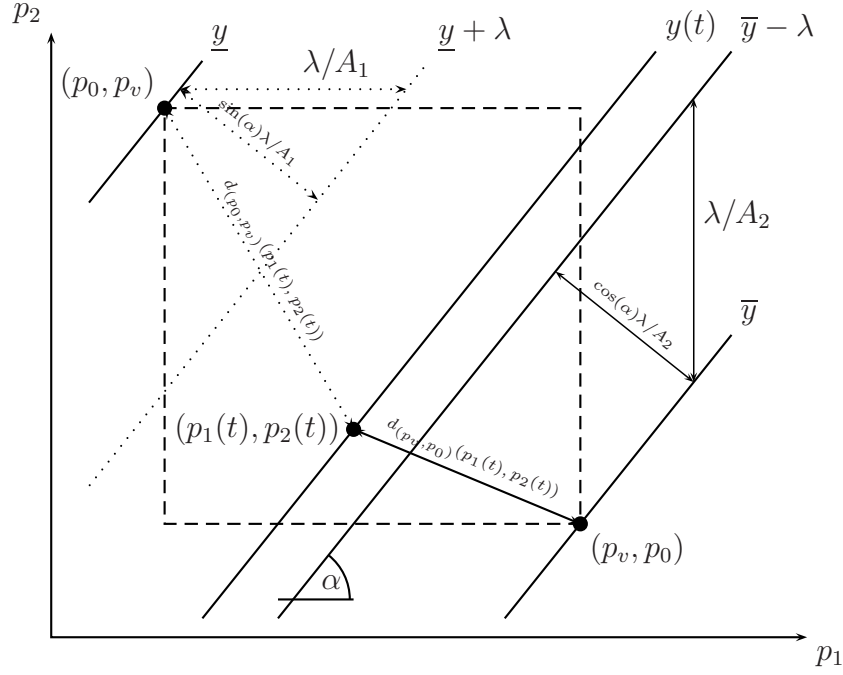
Figure 5: Geometric observation
