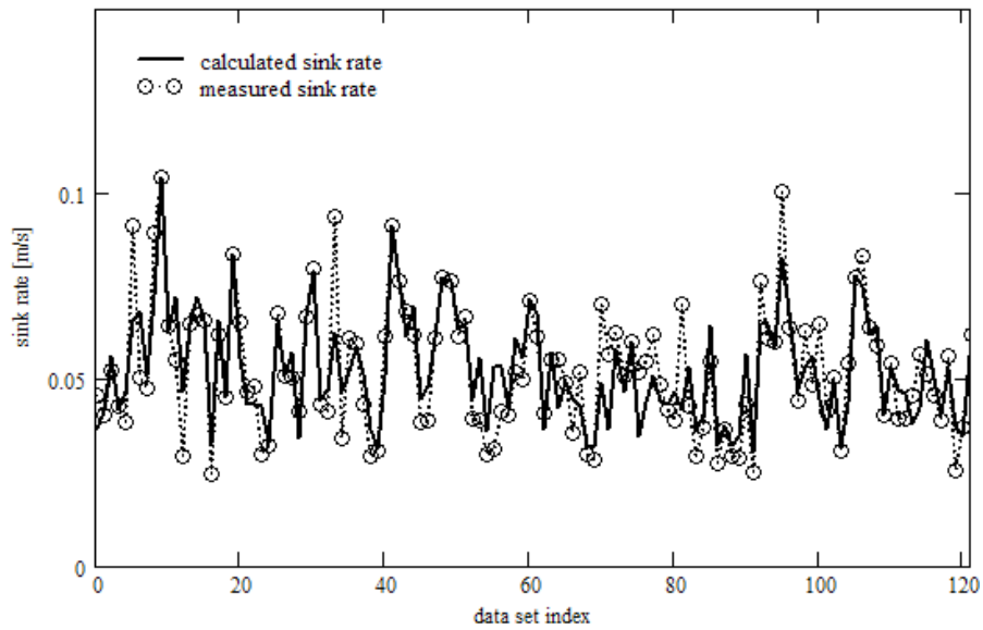
Fig. 7: Model output and measured particle sink rates (isolation material MD-K)
