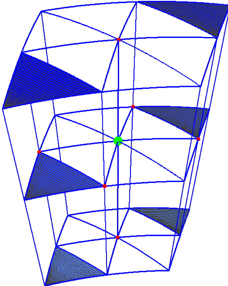
Figure 2.18: Refined double prism. Note that this macro has the same dof as the quadrilateral Q_2, P_1^{disc} element pair. The dof at the red points can be used to control the flux through the faces. This is necessary to fulfill the global LBB for discontinuous piecewise constant pressure. The dof at the green point can be used to fulfill the local LBB for the piecewise linear pressure. Unlike the Q_2, P_1^{disc} element pair it is not possible to define a bubble function which is different from zero on the whole top face and zero on all other faces. The same is true for the bottom face. The difficulties stem from the filled triangles. A piecewise linear function that is zero on the boundary of the whole quadrilateral is bound to be zero on the filled triangles. Nevertheless it is possible to control the flux through the whole face by the dof situated at the red point in the center of the face. The “bubble” is just a “tent” which is “flat” on the filled triangles.
