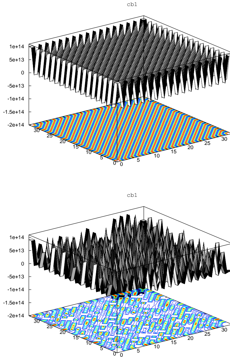
Figure 3.1: cb1 means checkerboard viscosity with patch size 1 \times 1 . As in all other cases the viscosity varies from 10^0 to 10^{14} from patch to patch. This profile is supposed to be the most unpleasant one for multigrid because a coarser grid could definitely not sample all jumps. The second plot shows the unsymmetrical version of cb1, the biggest jump is also 10^{14} but the others are randomized. The randomization was introduced because the results had been too good for this scheme. This fact, however, has not been changed by the randomization as we will see and explain later.
