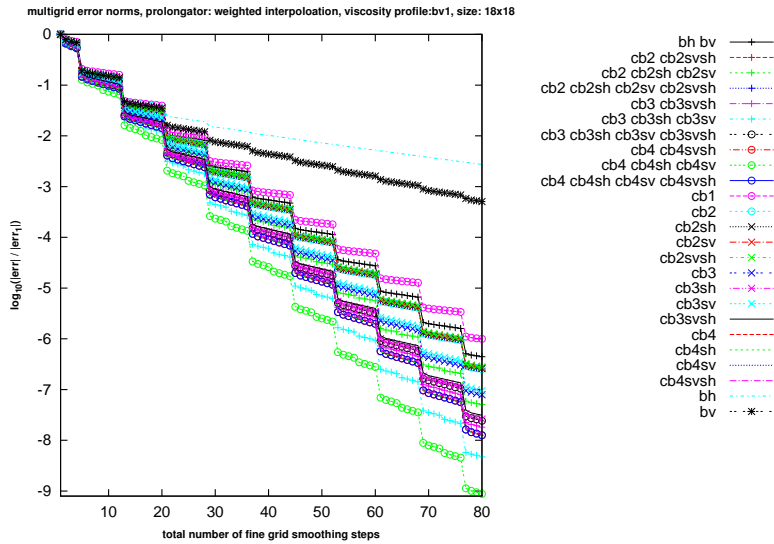
Figure 3.12: Error history. Please compare to Fig. 3.11! The error actually decreases after a multigrid step, although the residual plot seems to indicate the opposite.
