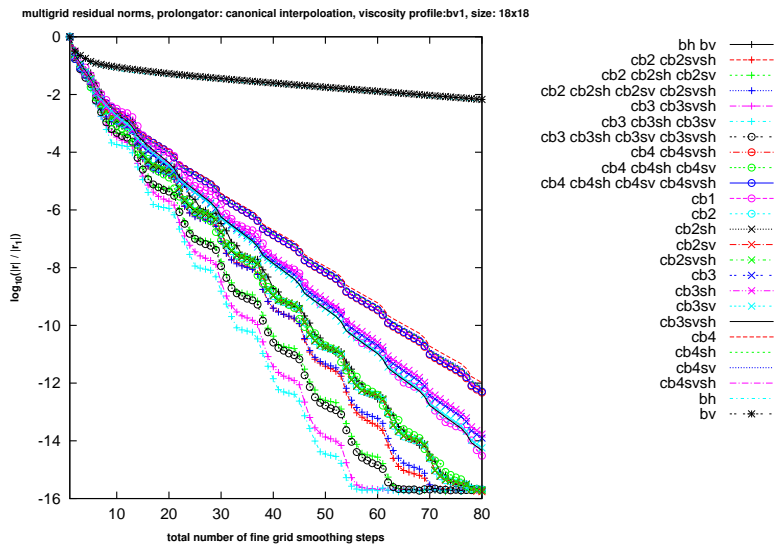
Figure 3.13: Residual history. Please compare to Fig. 3.14. The almost straight lines indicate that the number of pre and post smoothing steps is nearly optimal. This is, however, not true as the error history makes clear.
