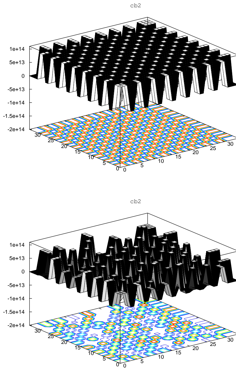
Figure 3.2: slightly increased patch-size to 2 \times 2 as the index 2 suggests. Bigger patches occur at the boundary due to the odd grid size
