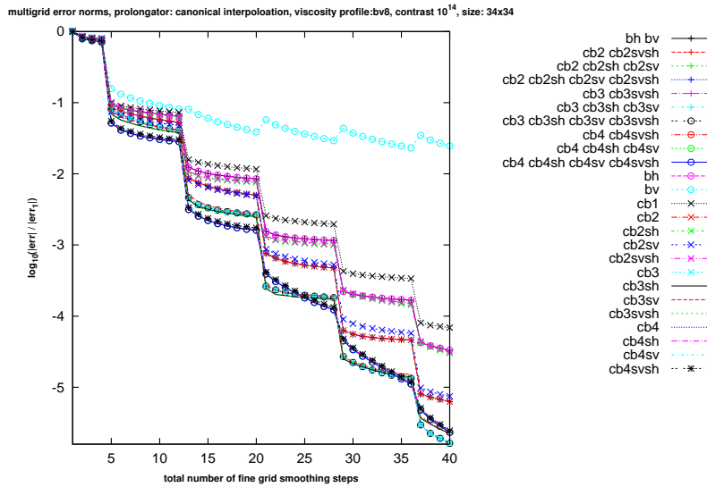
Figure 3.20: fine-grid error-history. The bv line-Jacobi smoother (cyan circles) has no benefit from the coarse-grid “corrections”. Surprisingly this does not happen for the first v-cycle and (only in this plot) never for the bh scheme. Note also the steep error drops after the coarse-grid correction and the almost level steps, where only the smoothers work.
