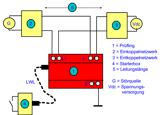
Figure 4 – Basic test setup for conducted RF-immunity
