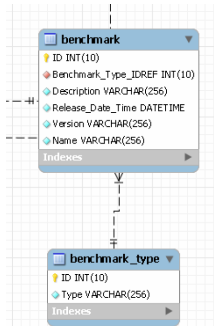
Figure 1: Excerpt from the ER-Model of the database
