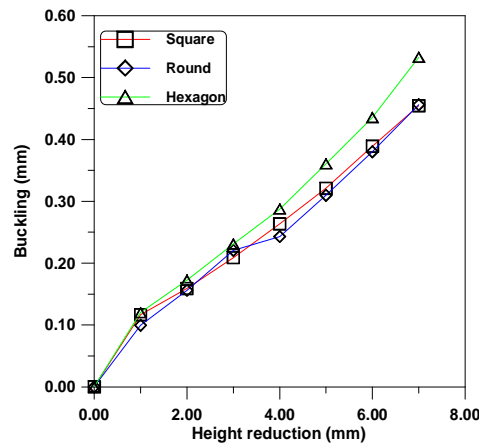
Fig.8 The influence of billets sectional shapes on upsetting buckling (at 1mm/sec punch velocity)
