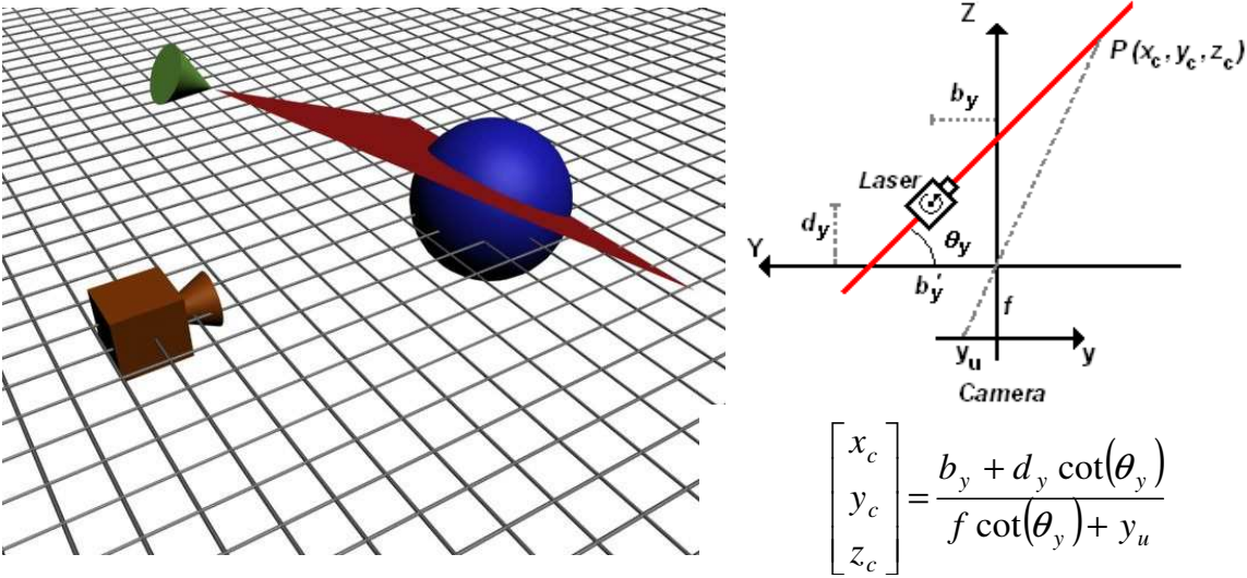
Fig. 4: Vision Sensor Mathematical Model
