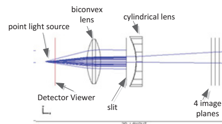
Fig. 3: ZEMAX 3D-Layout
