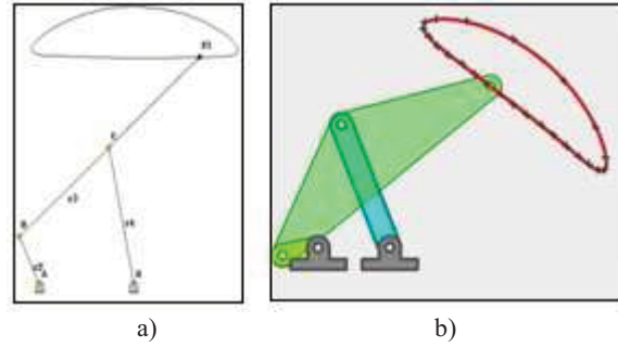
Fig. 6: Mechanisms, a) Hoekens; b) Burmester.
