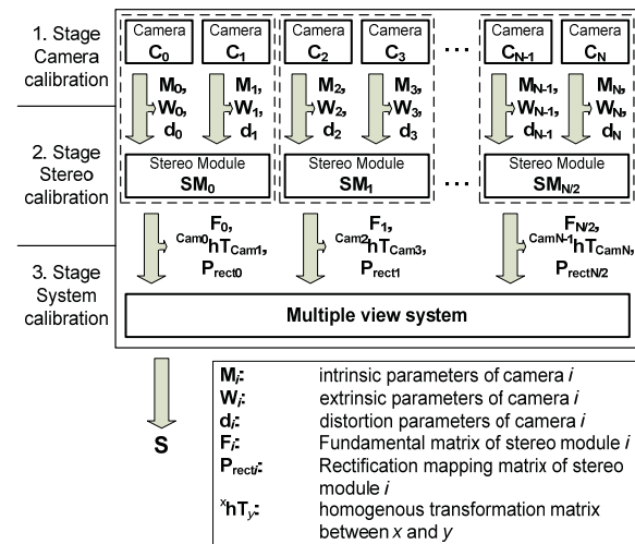
Fig. 5: Stereo modules calibration procedure workflow
