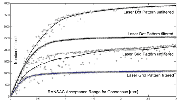
Fig. 6: Experimental results on accuracy and variation of different laser patters and filtering
