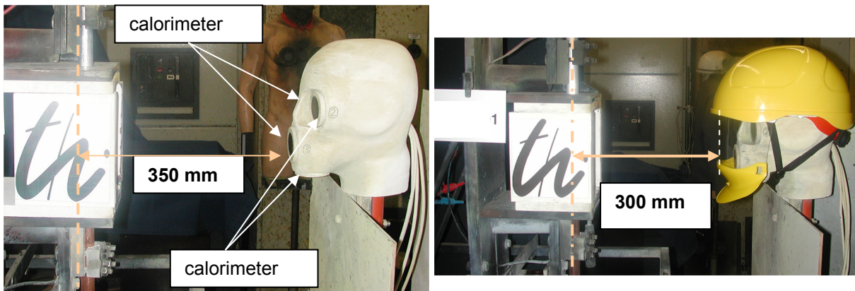
Fig. 1: Test set-up with test head equipped by calorimeters (left) and position of the test sample (example: visor-helmet combination, right)
