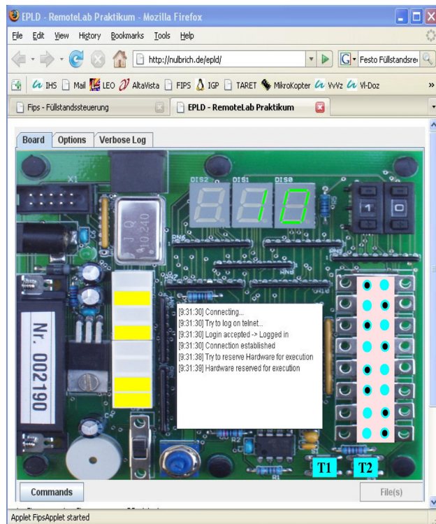
Figure 5. Web-interface of the Rapid Prototyping board
