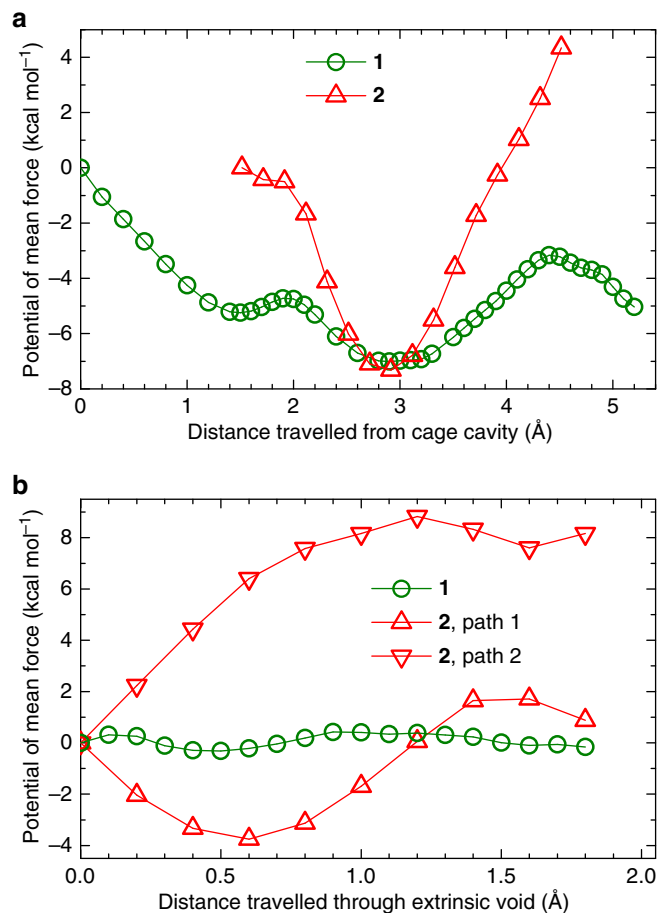
Figure 5 | Potential of mean force profiles of a water molecule diffusing in 1 and 2. The potential of mean force (PMF) profiles were plotted as a function of the reaction coordinate, which is the distance between the centre of mass (COM) of the water molecule and (a) the COM of the cage or (b) the COM of a cage window; the PMF at the starting position was arbitrarily set to zero. The results were obtained using solid-state classical molecular simulations.
