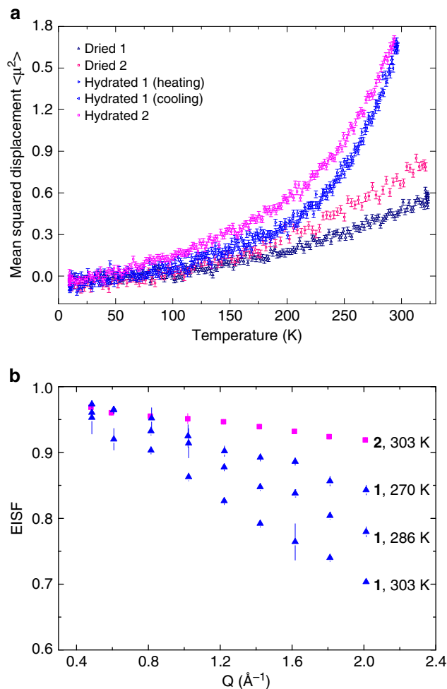
Figure 6 | Quasi-elastic neutron scattering measurements for cage salts 1 and 2. (a) Mean squared displacements with associated experimental error bars derived from the temperature-dependent normalized elastic scattering intensities of 1 and 2 from fixed window scan using the high-flux backscattering spectrometer (HFBS). (b) Elastic incoherent structure factor (EISF) of hydrated 1 (270, 286 and 303 K) and hydrated 2 (303 K) from the data measured on the Disk Chopper Spectrometer (DCS). Error bars indicate uncertainties derived from fitting the elastic and inelastic contributions to the experimental QENS intensities.
