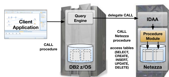
Figure 3: Stored Procedure Execution in Netezza
