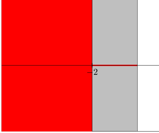
Figure 5: Theorem 7.2 (i) with \beta = 4 , \mu = 0 , \delta = 0 .
