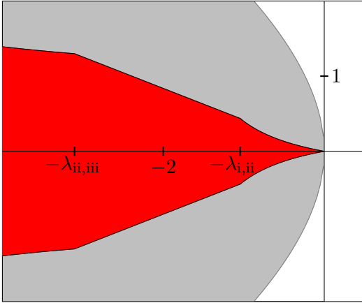
Figure 3: Theorem 6.2 (i), (ii), (iii) without Theorem 6.1 with k = 0.2 , \beta = 4 , \mu = 2.1 , \delta = 1.05 ; here \lambda_{i,ii} \approx 1.04 , \lambda_{ii,iii} \approx 3.10 , see Remark 6.6.
