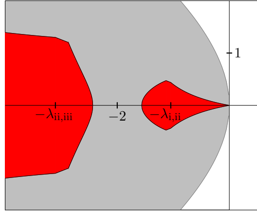
Figure 4: Theorem 6.2 (i), (ii), (iii) and Theorem 6.1 with k = 0.2 , \beta = 4 , \mu = 2.1 , \delta = 1.05 ; here \beta\delta > 4 , k > \frac{4}{\beta\delta} - 1 , \lambda_{i,ii} \approx 1.04 , \lambda_{ii,iii} \approx 3.10 , I_{0,\mu} \approx (1.12, 2.87) , I_0 \approx (1.56, 2.44) , see Re- mark 6.6.
