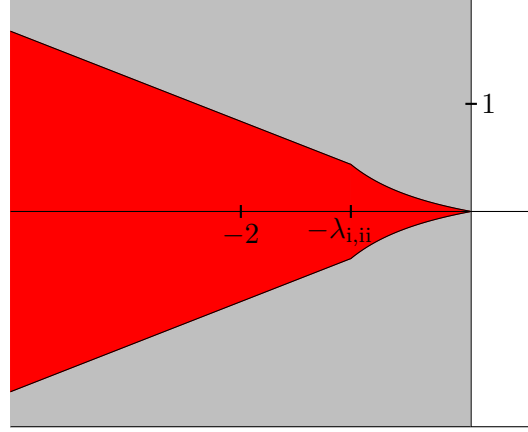
Figure 2: Theorem 6.2 (i), (ii) with k = 0.2 , \beta = 4 , \mu = 2.1 , \delta = 0 ; here \lambda_{i,ii} \approx 1.04 .
