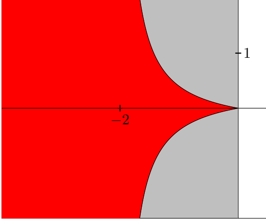
Figure 1: Theorem 6.2 (i) with k = 0.2 , \beta = 4 , \mu = 0 , \delta = 0 .
