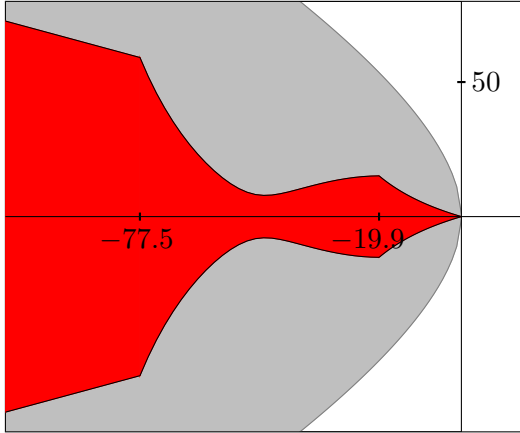
Figure 9: Example 8.3 for physical parameters E = 25 , C = 1 , K = 14 .
