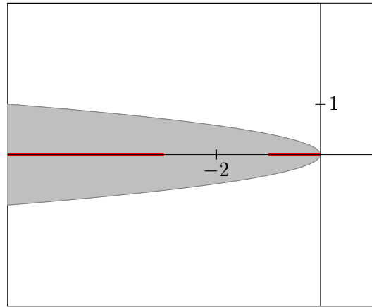
Figure 8: Theorem 7.2 (iii) with \beta = 4 , \delta = \frac{4}{3} ; here spectral gap in -I_0 = -I_{0,\mu} = (-3, -1) by Theorem 6.1, see Remark 6.6.
