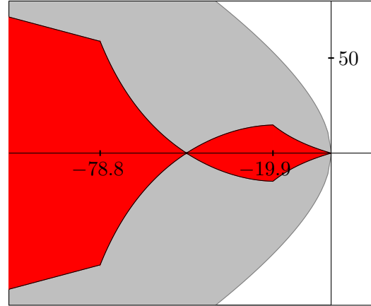
Figure 10: Example 8.3 for physical parameters E = 25 , C = \frac{10}{\pi^2} , K = 14 .
