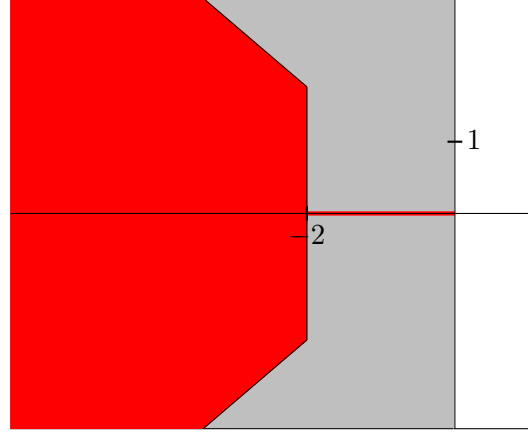
Figure 6: Theorem 7.2 (i), (ii) with \beta = 4 , \mu = 1.5 , \delta = 0 .
