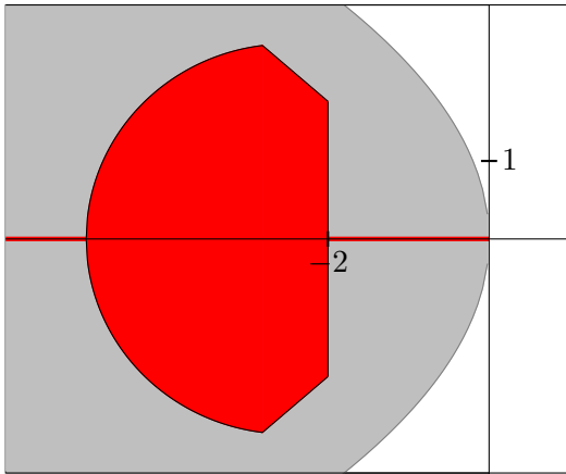
Figure 7: Theorem 7.2 (i), (ii), (iii) with \beta = 4 , \mu = 1.5 , \delta = 0.4 ; here k_\mu^2 = \frac{7}{9} < \frac{3}{2} = \frac{4}{\beta\delta} - 1 , I_0 = I_{0,\mu} = \emptyset , so no improvement by Theorem 6.1, see Remark 6.6.
