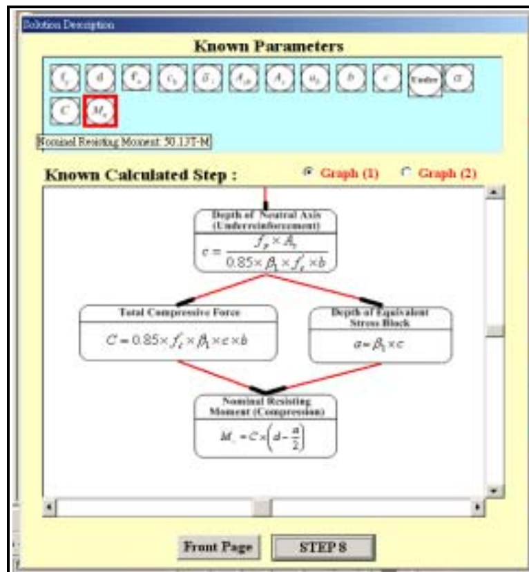
Figure 6. Answer evaluator
