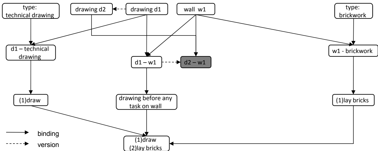
Figure 9: Affected relation becomes obsolete and a new version is required
