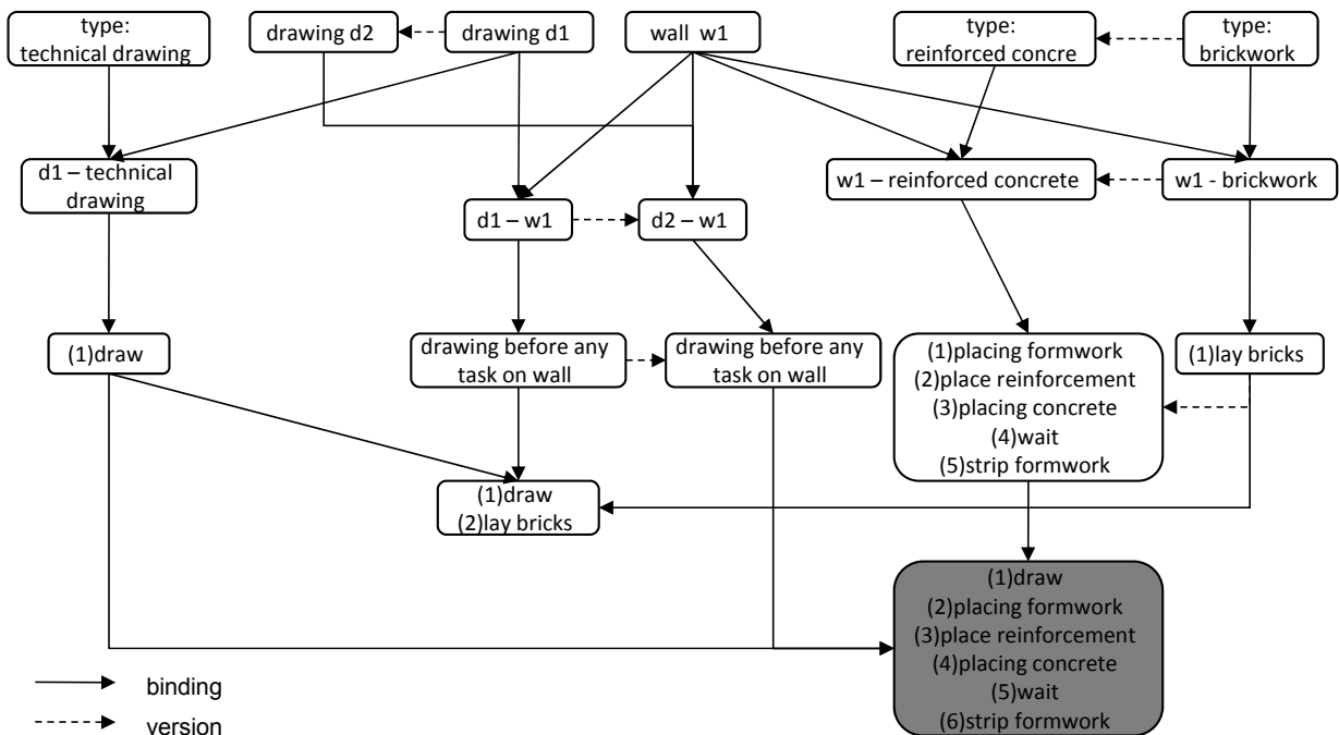
Figure 13: The new project task sequence
