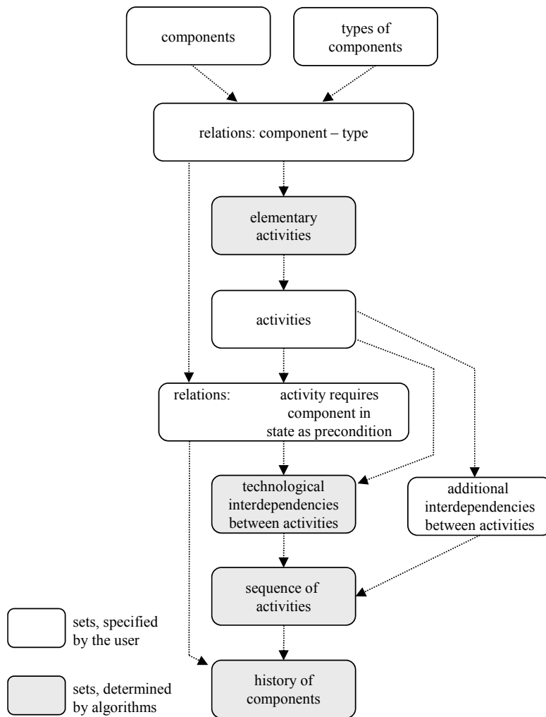
Figure 3: Specification and Computation of a Process Model for Engineering Construction Projects
