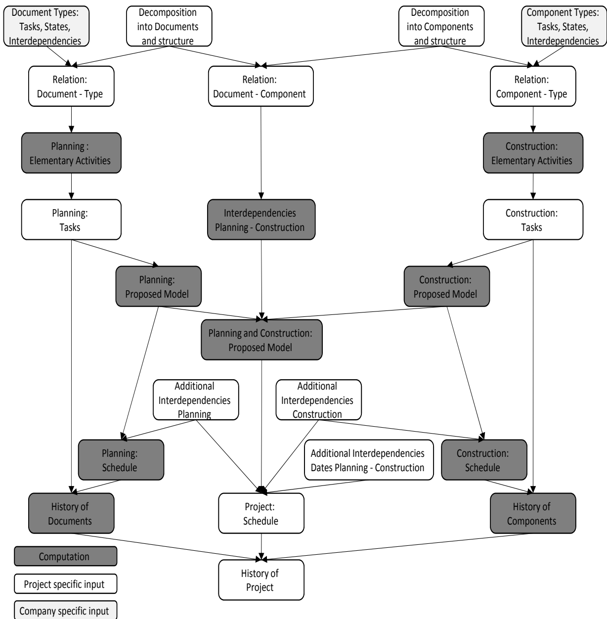
Figure 5: Specification and Computation of a complete Engineering Process Model
