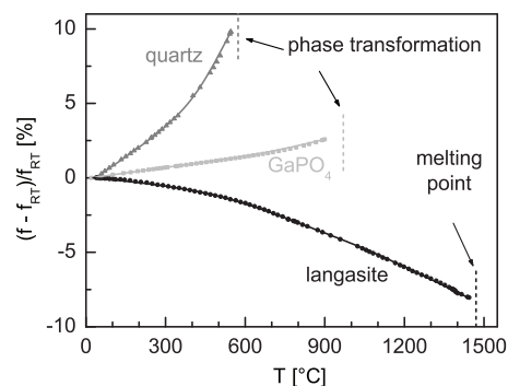
Figure 1. Temperature dependent resonance frequency f of piezoelectric crystals and related operation temperature limits. f_{RT} is the resonance frequency at room temperature. 35
