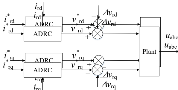
Figure 7. RSC control structure with ADRC. Figure 7. RSC control structure with ADRC.
