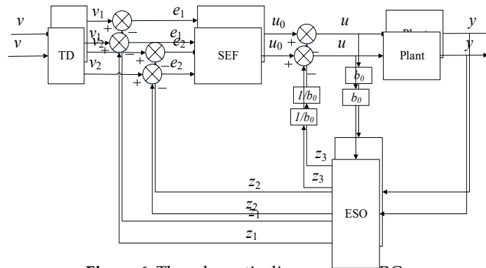
Figure 6. The schematic diagram of ADRC. Figure 6. The schematic diagram of ADRC.
