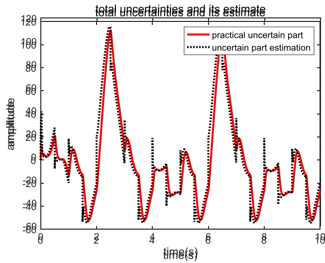
Figure 13. External disturbances and ESG prediction results.
