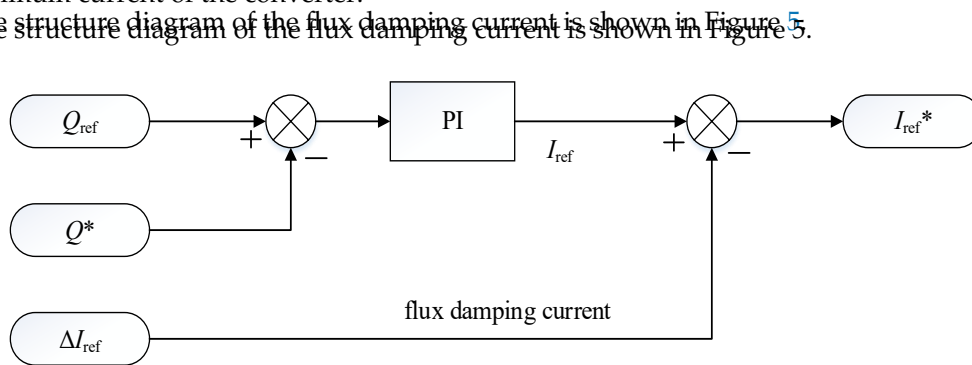
Figure 5. The schematic diagram of the flux damping current.
