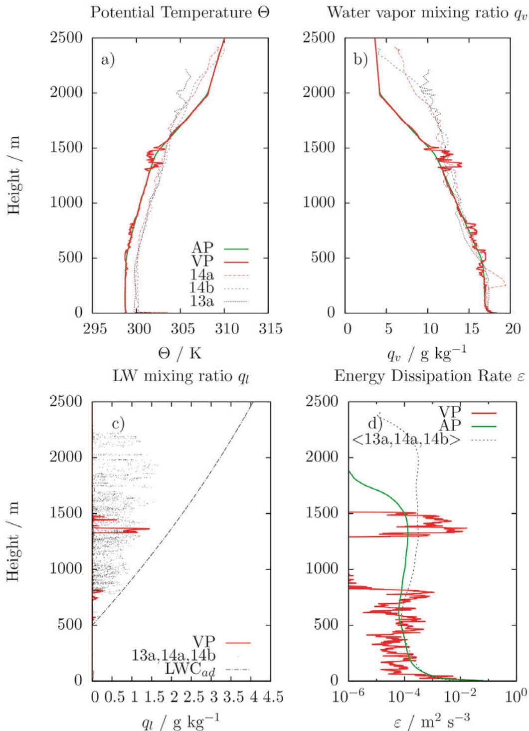
Figure 2: Vertical profiles of (a) potential temperature in K, (b) specific humidity in \text{g kg}^{-1} , (c) liquid water mixing ratio in \text{g kg}^{-1} , and (d) local energy dissipation rate in \text{m}^2 \text{s}^{-3} as a function of height above sea level in m for (temporally and horizontally) averaged LES profiles (AP), virtual ACTOS-profiles measured in the LES domain (VP), and averaged ACTOS profiles sampled during three flights (April 13, 14a, and 14b, 2011) of the CARRIBA campaign. The adiabatic liquid water mixing ratio (cloud base at 500 m with T = 21^\circ\text{C} ) has been added to (c) for reference. All three CARRIBA profiles (13, 14a, 14b) have been averaged to one profile in (d).
