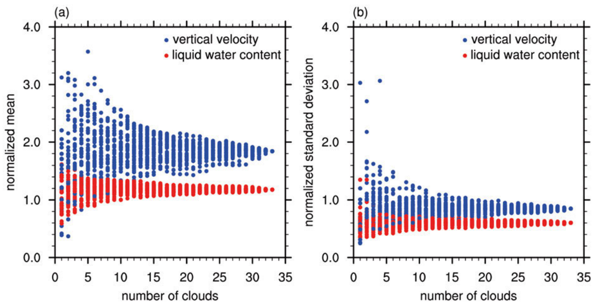
Figure 8: Normalized mean (a), and normalized standard deviation (b) as a function of the number of analyzed clouds for liquid water content (red circles) and vertical velocity (blue circles). 50 randomly chosen orders of 33 examined clouds are displayed. Values are normalized by the corresponding two-dimensional mean (see text for more details on the normalization).
