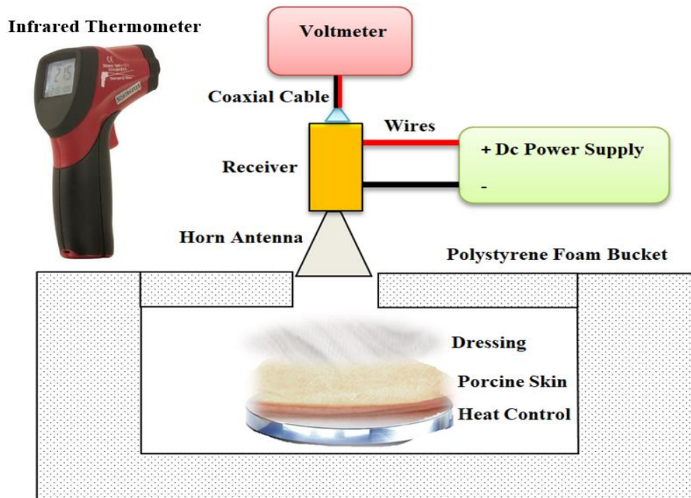
Figure 3. Experimental setup for the emissivity measurements of the porcine skin samples. A digital voltmeter is used to measure the output voltage level of the samples and a thermocouple and an infrared thermometer are used to measure the thermodynamic temperature of the samples.
