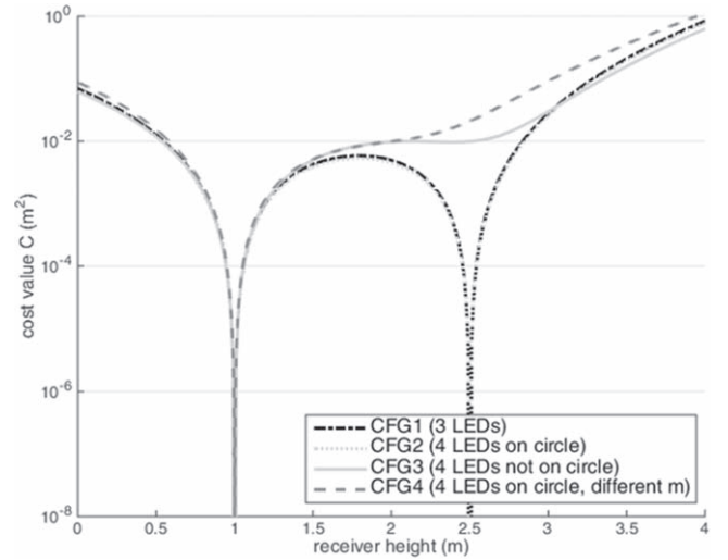
Figure 2. Cost function for the different LED configurations for (5.5, 7.5, 1).
