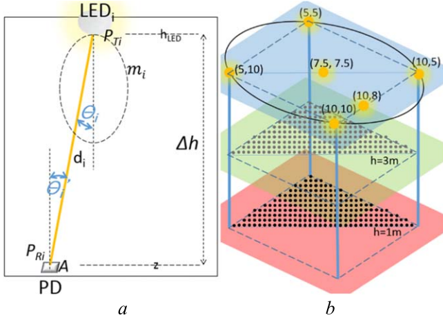
Figure 1. (a) Definition of configuration parameters and (b) considered setup with indication of the involved LED locations and evaluation grid.
