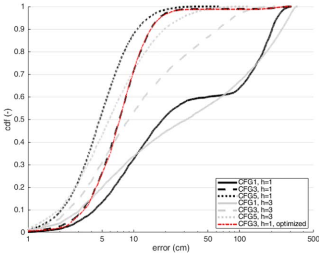
Figure 3. Cdf of errors inside triangle of figure 1(b) for CFG1-3-5 at h = 1 and 3 m.
