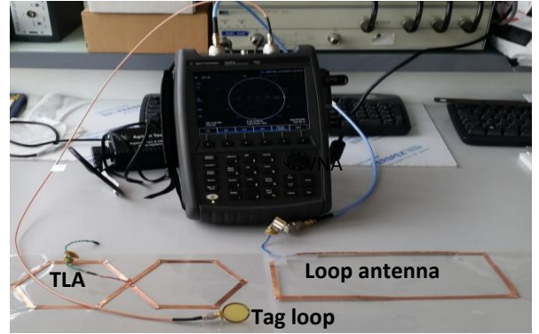
Fig.6 Experiment setup
