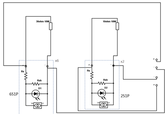
Figure 9: Solar Panel test layout
