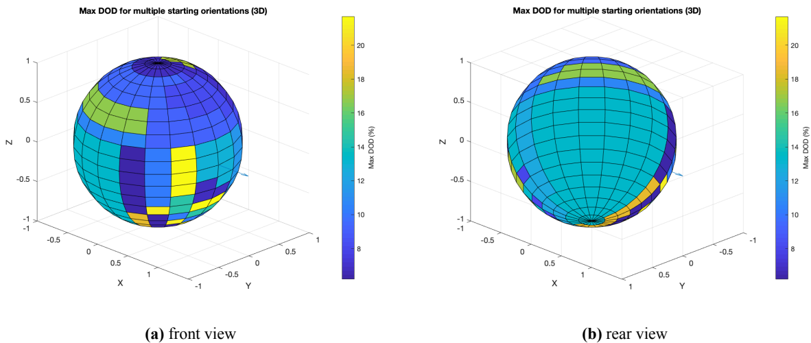
Figure 5: Maximum Battery DOD for each attitude
