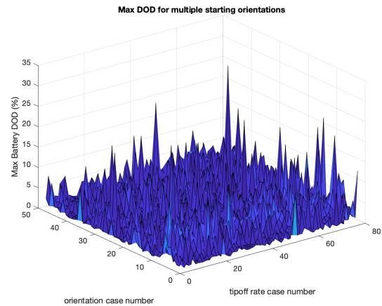
Figure 6: Maximum Battery DOD for each case
