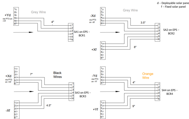
Figure 3: Solar Panel Wiring Diagram
