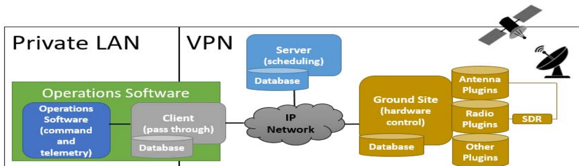
Figure 1: SATRN Architecture
