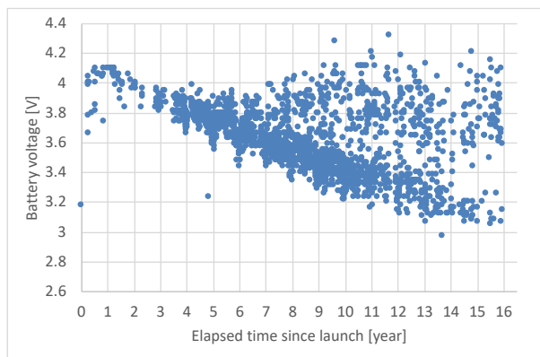
Figure 5: 15-years trend of battery voltage
