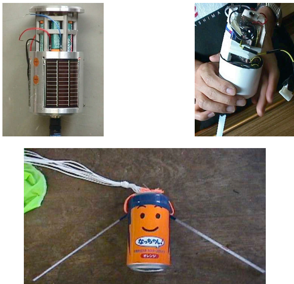
Figure 1: The University of Tokyo's three CanSats from 1999 (the first year of ARLISS)
