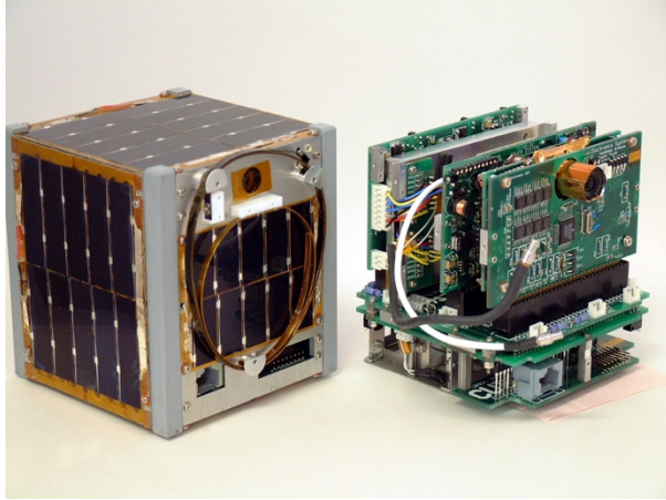
Figure 2: The University of Tokyo's CubeSat-XI (left: external appearance, right: internal structure)
