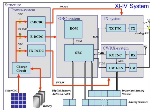
Figure 4: System block diagram of XI-IV
