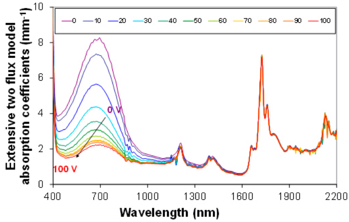
Figure 18. Voltage dependence of the extensive two flux model absorption coefficients of the SPD
