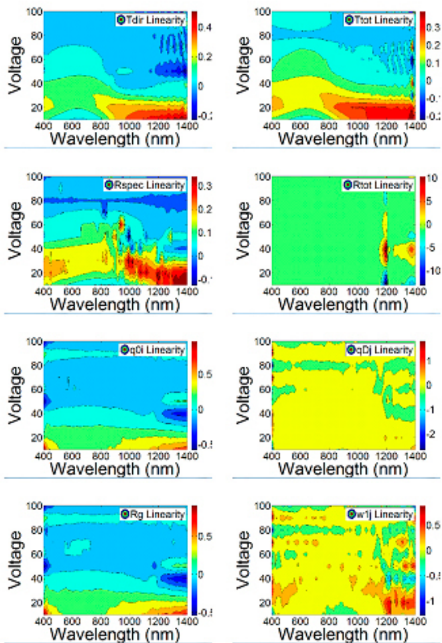
Figure 19. Voltage dependence of the linearity of the parameters showing contrast differences in the SPD
