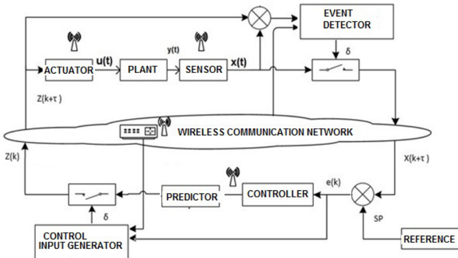
Figure 2. Structure of the WNSC system implemented
