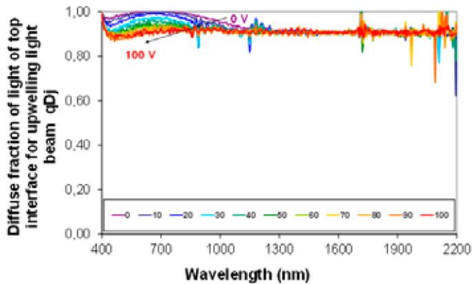
Figure 16. Voltage dependence of q_D^j , the diffuse fractions of light of the SPD for upwelling light beam “j” at the top interface “D”
