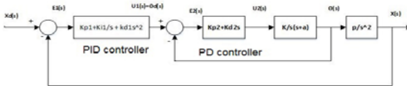
Figure 4. Block diagram of the BB system implemented
