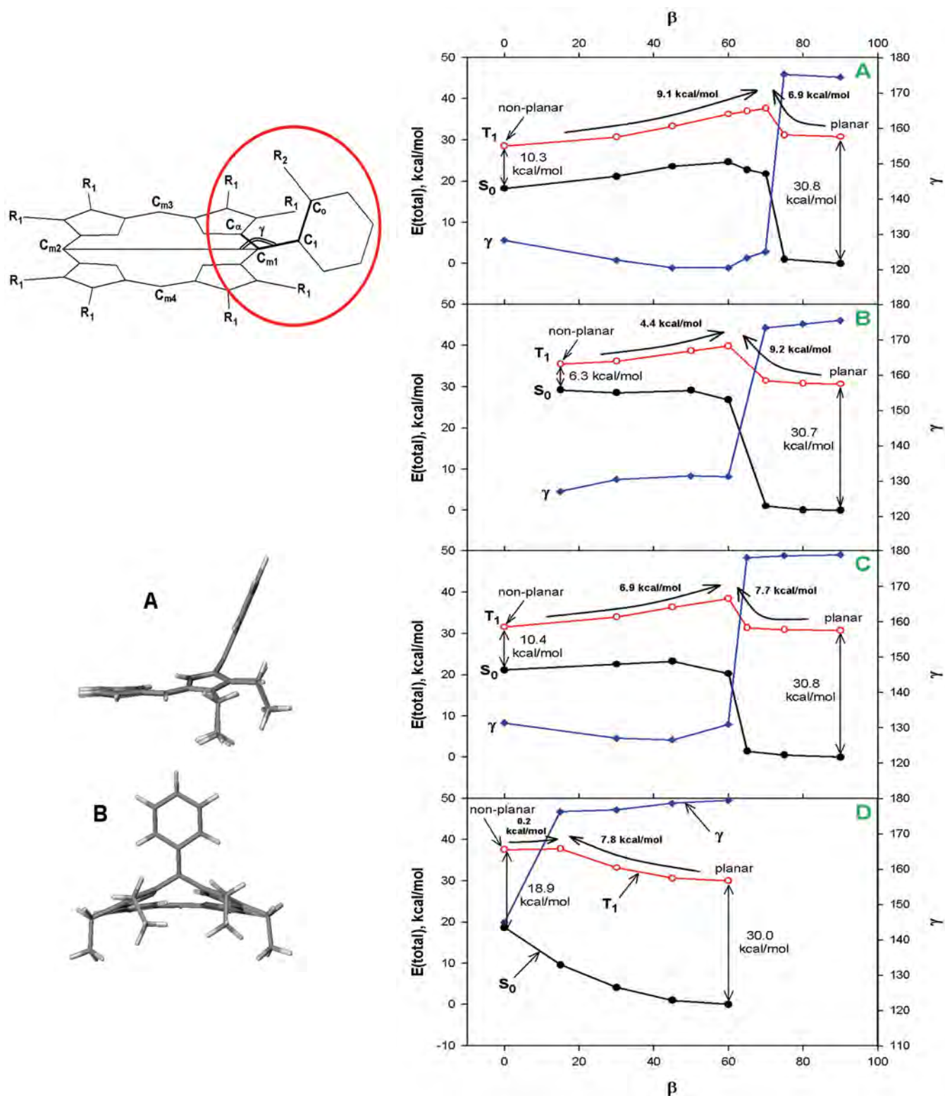
Figure 8. Left (Top): Structure elements for the compounds under consideration OEP-Ph: R_1=C_2H_5 , R_2=H ; OEP-Ph( o -CH 3 ): R_1=C_2H_5 , R_2=CH_3 . In calculations alkyl groups on the pyrroles that are far from the phenyl ring were substituted by hydrogens. Dihedral angle \beta is formed by the atoms C_\alpha-C_{m1}-C_1-C_0 (marked with bold lines). Left (A, B): The non-planar conformation of 5Ph-OEP molecule in T_1 state depicted from two different sides (A, B). This conformation corresponds to the maximal conjugation of the phenyl ring with the porphyrin macrocycle ( \beta \sim 0^\circ ). Calculations were performed for structures with alkyl groups on the pyrroles distant from the phenyl ring substituted by hydrogens. Right: Theoretical dependence of the total energies, E(\text{total}) , for the excited T_1 (red curve, open circles) and ground S_0 (black curve, filled circles) states as well as the angle \gamma value (blue curve, filled diamonds) on the dihedral angle \beta : (A) - OEP-Ph (compound 10, Figure 1); (B) - OEP-Ph( o -CH 3 ) (compound 18, Figure 1); (C) - OMP-Ph; (D) - Porphyrin- meso -Ph (P-Ph). The energies of the ground S_0 state (black curves, filled circles) were calculated at the molecular geometry of the excited T_1 state. It means that the vertical energy gap \Delta E_{\nu}(T_1-S_0) corresponds to the energy difference between the corresponding T_1 and S_0 curves for every compound. The total energy of the ground S_0 state for planar conformations was taken to be E(S_0) = 0 in all cases. The values of the \Delta E_{\nu}(T_1-S_0) energy gap for planar and nonplanar conformations, as well as the heights of the barriers of conformational transformations, are shown.
