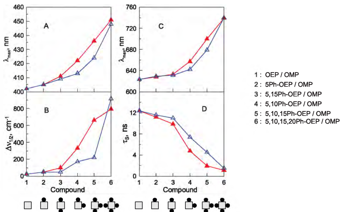
Figure 6. Correlation dependences of steric interactions for meso -phenyl substituted octaethylporphyrins (OEP, \blacktriangle ) and octamethylporphyrins (OMP, \blacktriangle ) reflecting changes of spectral-kinetic parameters upon sequential increase of number (and position) of meso -phenyl rings: \lambda_{\max} of Soret band in absorption (A); \Delta\nu_s , Stokes shift (B); \lambda_{\max} of the fluorescence band (C); fluorescence decay values \tau_s in non-degassed solutions (D). Pictograms are the same as in Figure 5.
