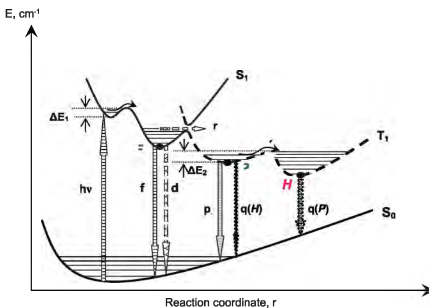
Figure 7. Energetic scheme of potential surfaces describing ground S_0 and locally excited S_1 and T_1 electronic states as well as photoinduced electronic transitions between these states for meso -phenyl substituted octaalkylporphyrins in liquid solutions at ambient temperature. \Delta E_1 and \Delta E_2 are the potential barriers for conformational rearrangements of non-planar porphyrin macrocycle. The rate constants of radiative and non-radiative transitions are denoted as follows: (f) – fluorescence S_1 \rightarrow S_0 ; (d) – internal conversion S_1 \rightarrow S_0 ; (r) – intersystem crossing S_1 \rightarrow T_1 ; (p) – phosphorescence T_1 \rightarrow S_0 ; q(H) and q(P) – intersystem crossing transitions T_1 \rightarrow S_0 from the triplet to the ground state for nonequilibrium (H) and equilibrium (P) conformations of the tetrapyrrole macrocycle.
