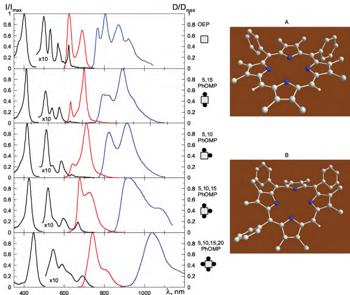
Figure 5. Normalized absorption (black), fluorescence (red) and phosphorescence (blue) spectra in toluene at ambient temperature for (from top to down) OEP; 5,15Ph-OEP; 5,10Ph-OEP; 5,10,15Ph-OEP; 5,10,15,20Ph-OEP. Pictograms on the right present structural features of the compounds under study with increasing number of meso -phenyl substituents, black circles indicate meso -phenyl rings. Right: Structures of sterically hindered meso -phenyl substituted 2,3,7,8,12,13,17,17-octamethylporphyrins, (A) for 5,10-diphenyl OMP and (B) for 5,10,15-triphenyl OMP, on the basis of X-Ray STOE IPDS data (friendly given by Profs. P. Stuzhin, A. Semeikin and O. Koifman).
