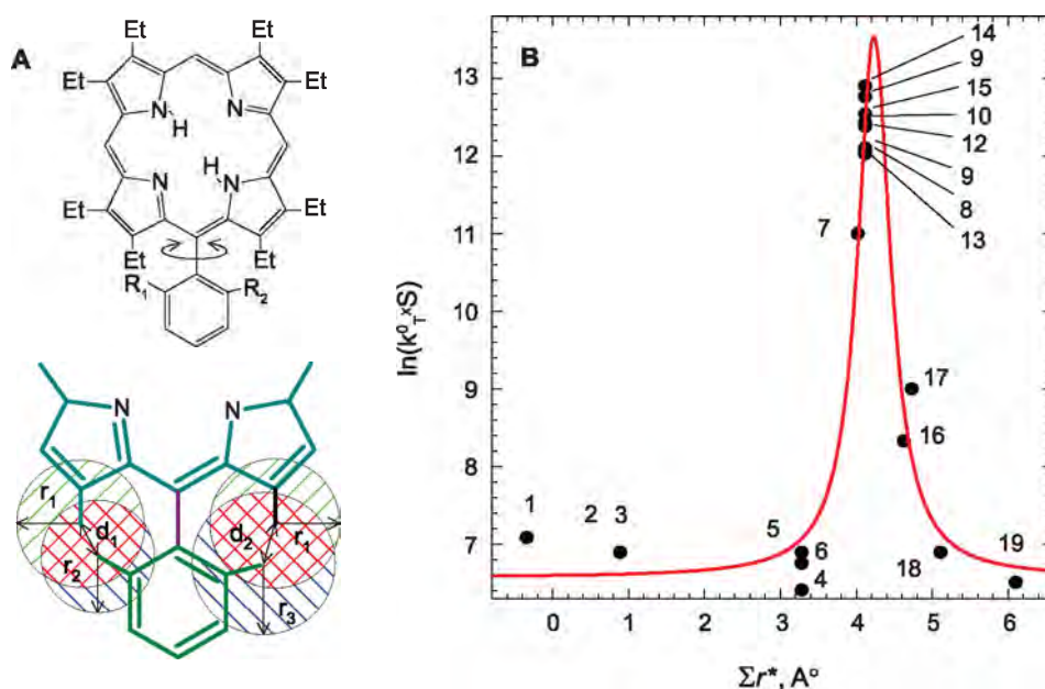
Figure 4. Schematic representation of the «apparent overlap» of interacting flanking groups in a crowded transition state (A) and the correlative dependence (B) of the triplet state deactivation rate constants k_T^0 on the overlap geometrical parameter ( \Sigma r^* ), \ln(k_T^0) = \ln(1/\tau_T^0) = f(\Sigma r^*) , for the compounds being studied in toluene at 295 K. (A): The inset shows a schematic structural presentation of the effective Van der Waals radii ( r_i ) for interacting substituents, intercenter distances d_1 , d_2 and corresponding substituent bond lengths in the porphyrin macrocycle and in the ortho -positions of the phenyl ring solid lines for the hypothetical coplanar arrangement of the porphyrin macrocycle and the phenyl ring planes (HyperChem optimization). The contributions to \Sigma r^* in meso -aryl substituted porphyrins have been calculated using equation \Sigma r^* = (r_{X1} + r_{X2}) - d_X + (r_{Y1} + r_{Y2}) - d_Y (B): Numbers 1–19 correspond to compounds with the chemical structure shown in Figure 1.
