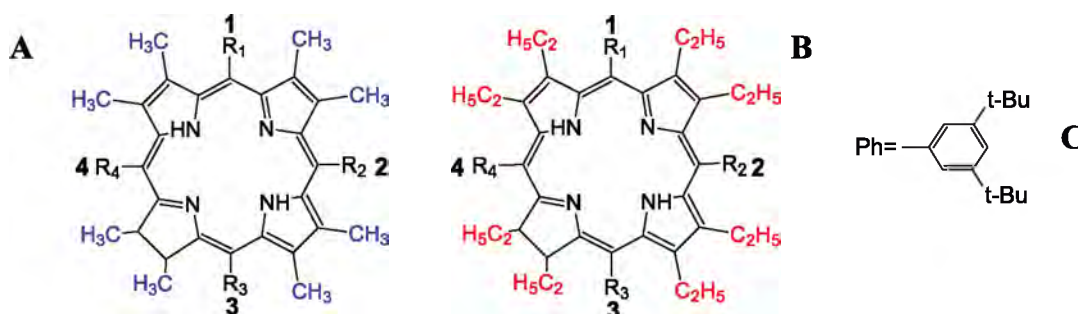
Figure 2. Chemical structures and abbreviations of octamethylporphyrin (A, OMP) and octaethylporphyrin (B, OEP) molecules and their meso -phenyl substituted (Ph) derivatives. OEP / OMP: R_1=R_2=R_3=R_4=H ; 5-PhOEP / OMP: R_1=Ph, R_2=R_3=R_4=H ; 5,15Ph-OEP / OMP: R_1=R_3=Ph, R_2=R_4=H ; 5,10Ph-OEP / OMP: R_1=R_2=Ph, R_3=R_4=H ; 5,10,15Ph-OEP / OMP: R_1=R_2=R_3=Ph, R_4=H ; 5,10,15,20Ph-OEP / OMP: R_1=R_2=R_3=R_4=Ph .
