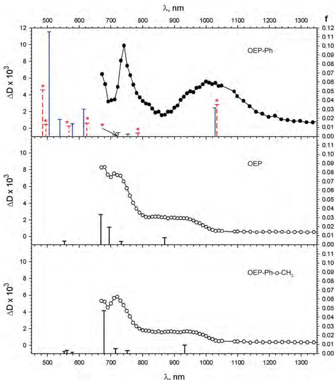
Figure 9. Experimental T_1 \rightarrow T_n absorption spectra of OEP-Ph (A), OEP (B) and OEP-Ph( o -CH 3 ) (C). They are compared with the calculated T_1 \rightarrow T_n absorption spectra of OEP-Ph in non-planar, planar and saddle-shaped conformation. The calculated transitions of the non-planar conformation of OEP, corresponding to the non-planar conformation of OEP-Ph, but without the phenyl are marked by asterisk. One of the transitions, calculated for this molecule, practically coincide by its energy and intensity with the corresponding transition in OEP-Ph. An arrow marks its position. Note that calculations were performed for structures without alkyl groups on the pyrroles distant from the phenyl ring.
