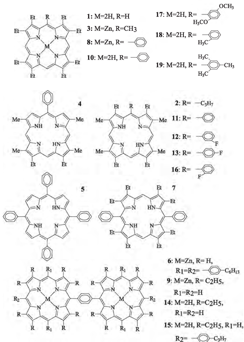
Figure 1. Chemical structures and abbreviations for a series of porphyrins and their phenyl bridged chemical dimers with a controllable structure of meso -phenyl substituents: 1 = octaethylporphyrin, OEP; 2 = etioporphyrin II, EPII-Pr; 3 = Zn-octaethylporphyrin, ZnOEP- CH_3 ; 4 = tetramethyldiethylporphyrin, TMDE-Ph; 5 = tetraphenylporphyrin, TPP; 6 = chemical dimer of Zn-tetra-hexylphenylporphyrin, ZnHTPP 2 ; 7 = 5,15-phenyl OEP, Ph-OEP-Ph; 8 = ZnOEP; 9 = chemical dimer (ZnOEP) 2 -Ph; 10 = OEP-Ph; 11 = EPII-Ph; 12 = EPII-Ph( m -F); 13 = EPII-Ph( p -F); 14 = chemical dimer OEP-Ph-OEP; 15 = chemical dimer (PrPh) 2 -(OEP) 2 -Ph; 16 = EPII-Ph( o -F); 17 = OEP-Ph(OCH 3 ) 2 ; 18 = OEP-Ph( o -CH 3 ); 19 = OEP-Ph(CH 3 ) 3 .
