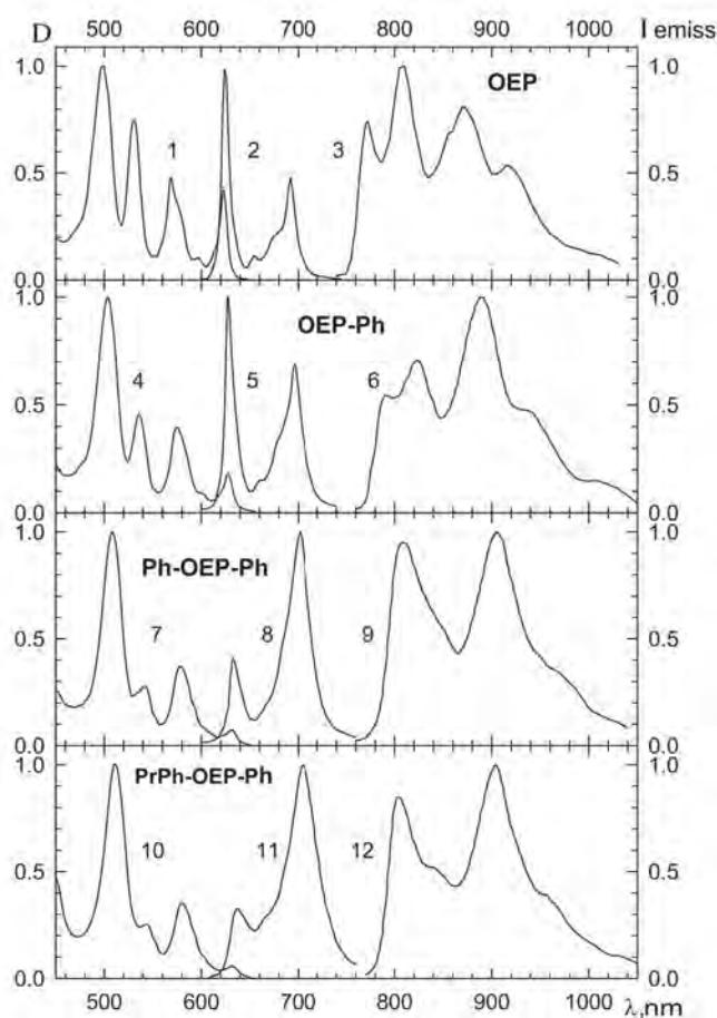
Figure 3. Absorption (1, 4, 7, 10) and fluorescence (2, 5, 8, 11) spectra in toluene at 295 K and phosphorescence spectra 3, 6, 9, 12 in methylcyclohexane-toluene mixture 6:1 at 77 K for porphyrins with mono- and di- meso -aryl substitution and their chemical dimer: OEP (1, 2, 3); OEP-Ph (4, 5, 6); Ph-OEP-Ph (7, 8, 9); and PrPh-OEP-Ph (10, 11, 12).
