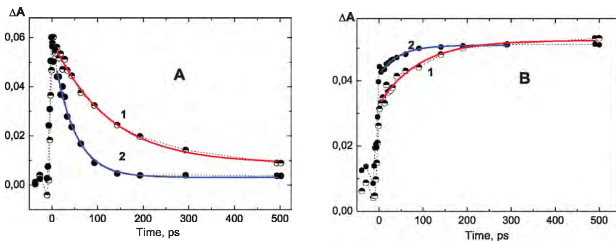
Figure 11. Kinetics of decay of transient absorption for OEP-Ph( o -NO 2 ) molecule (A, \lambda_{reg} = 480 nm,) and radical-ion pair absorption rise (B, \lambda_{reg} = 800 nm) in toluene (1) and dimethylformamide (2) at 295 K.
