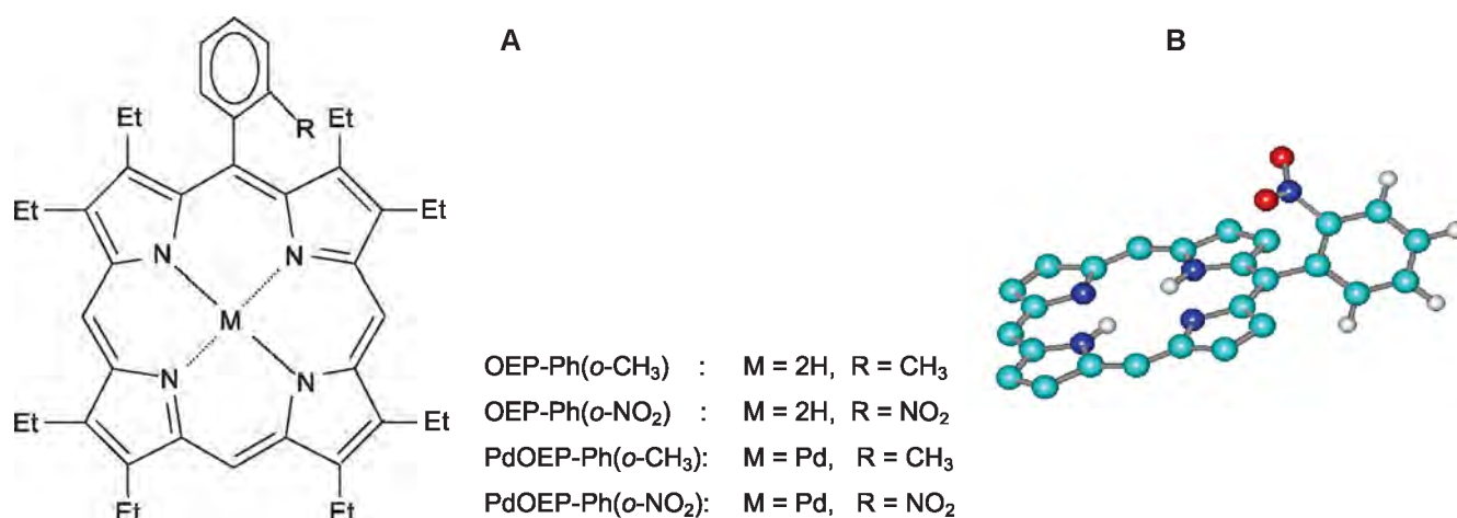
Figure 10. (A) Structural formulas of molecules studied and their abbreviations: 5-( ortho -methylphenyl)-2,3,7,8,12,13,17,18-OEP-Ph( o -CH 3 ); 5-( ortho -nitrophenyl)-2,3,7,8,12,13,17,18-octaethylporphyrin, OEP-Ph( o -NO 2 ); 5-( ortho -methylphenyl)-2,3,7,8,12,13,17,18-octaethylporphyrinato-Pd(II), PdOEP-Ph( o -CH 3 ); 5-( ortho -nitrophenyl)-2,3,7,8,12,13,17,18-octaethylporphyrinato-Pd(II), PdOEP-Ph( o -NO 2 ). (B): Optimized (HyperChem 4.0, semiempirical AM1 and PM3 methods) structure of octaethylporphyrin with NO 2 group in ortho -position of meso -phenyl. For clarity, bulky C 2 H 5 substituents in the β-positions of the pyrrole rings are omitted. Synthesis, purification, and characterization of these compounds were performed by Dr. A. Shulga. [77,78]
