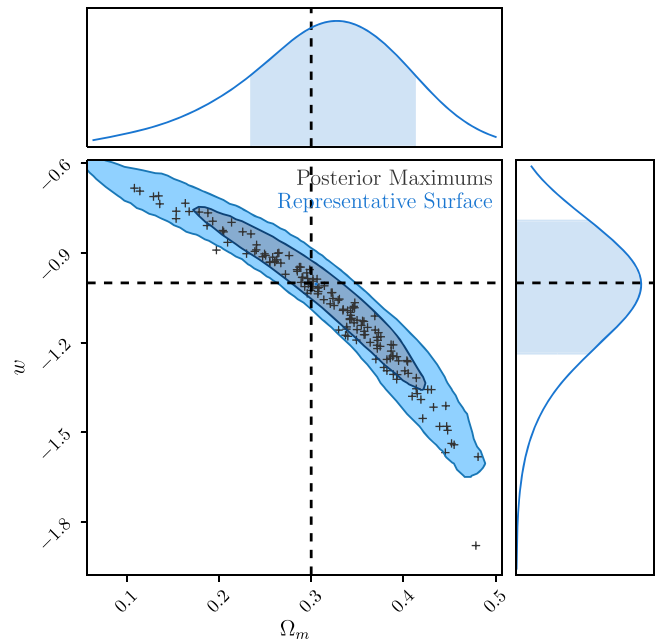
Figure 7. Maximal posterior points for 100 realizations of supernova data with the flat w CDM model, with a representative contour from a single data realization shown for context. The well-known banana-shaped contour is recovered, with the marginalized distributions in \Omega_m and w shown to recover input cosmology. For contours that are non-Gaussian due to the curved degeneracy between \Omega_m and w , the marginalized distributions can provide misleading statistics where maximum marginalized distribution can disagree with the maximum likelihood in multiple dimensions. For our contours, the non-Gaussianity is small, and the marginalized distributions still provide a valuable metric. The recovered posterior maxima show the same degeneracy direction as the representative surface and scatter around the truth values input into the simulation, which are shown with dashed lines.
