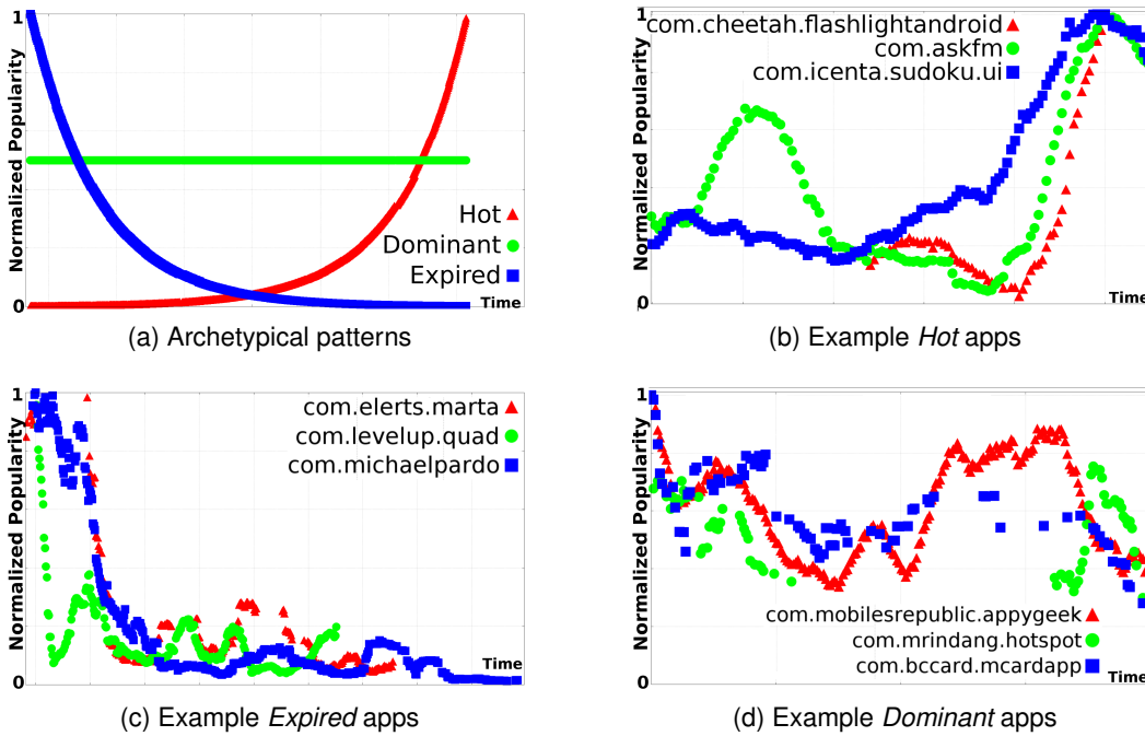
Fig. 4. Archetypical trend patterns and example applications following these patterns.
