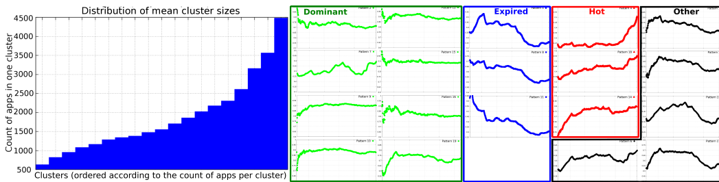
Fig. 8. Distribution of cluster sizes and consensus of the clusters found grouped with respect to their closest archetypical pattern.
