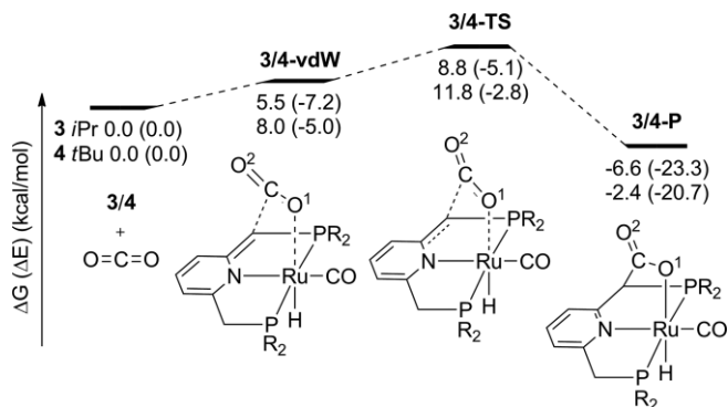
Figure 2. Relative \omega B97X-D/6-311G(d,p) Gibbs free energies (energy in brackets) in \text{kcal mol}^{-1} for the reaction of \text{CO}_2 and 3/4 .
