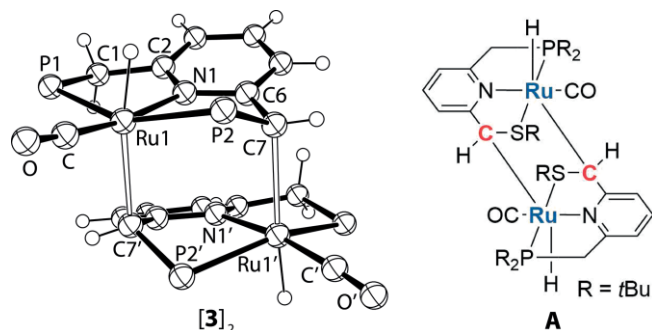
Figure 4. Two examples of dimeric MLC complexes. Left: molecular X-ray structure of [\mathbf{3}]_2 (displacement ellipsoids are set at 50% probability, isopropyl groups on the phosphorus are omitted for clarity). [12] Selected bond lengths [Å]: Ru1-C7' 2.409(7), Ru1'-C7 2.403(7), P2-C7 1.797(6), C6-C7 1.456(8), C1-C2 1.489(9), C1-P1 1.842(6), P2'-C7' 1.803(6), C6'-C7' 1.449(8), C1'-C2' 1.55(1), C1'-P1' 1.843(6). Right: Milstein's Ru(PNS) dimer A . [18] Blue: Lewis acid; red: Lewis base.
