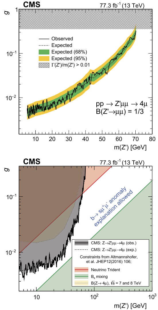
Fig. 6. Top: Expected and observed 95% CL limits on the gauge coupling strength g as a function of m(Z') . The dashed black curve is the expected upper limit, with one and two standard-deviation bands shown in green and yellow, respectively. The solid black curve is the observed upper limit. The B(Z' \rightarrow \mu\mu) = 1/3 is used to derive the upper limits. The hatched area shows the region where the narrow width approximation is no longer valid. Bottom: comparison with other experiments sensitive to the same parameter space, with shaded regions being excluded as described in the text. These three constraints are adapted from Ref. [13].
